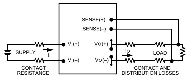
Figure 21. Effective Circuit Configuration for Single-Module Remote-Sense Operation
