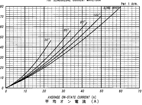
AVERAGE ON-STATE POWER DISSIPATION for SINUSOIDAL CURRENT WAVEFORM
