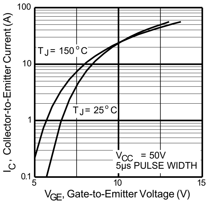
Figure 5c. Typical Transfer Characteristics
