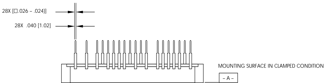
Figure 8b. Package Outline and Mechanical Specifications
