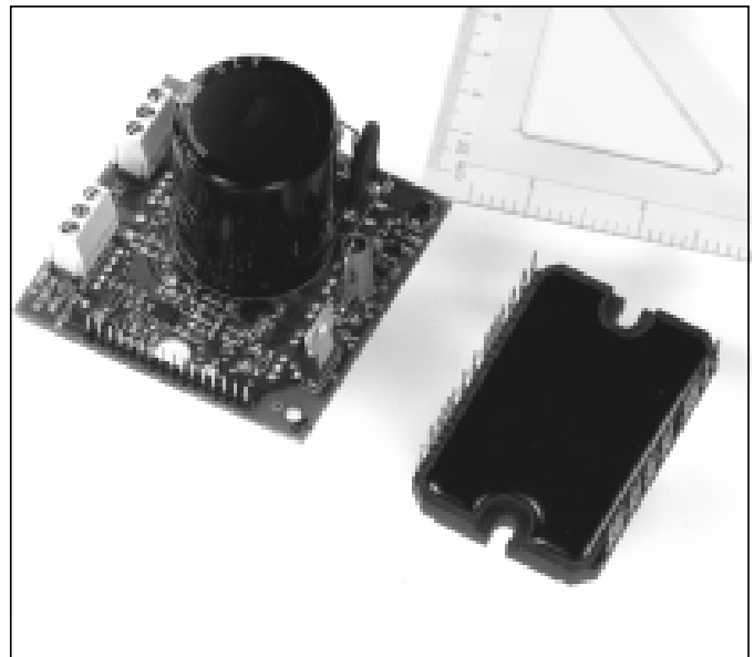
Figure 3. IRPT1060C POWIRTRAIN
