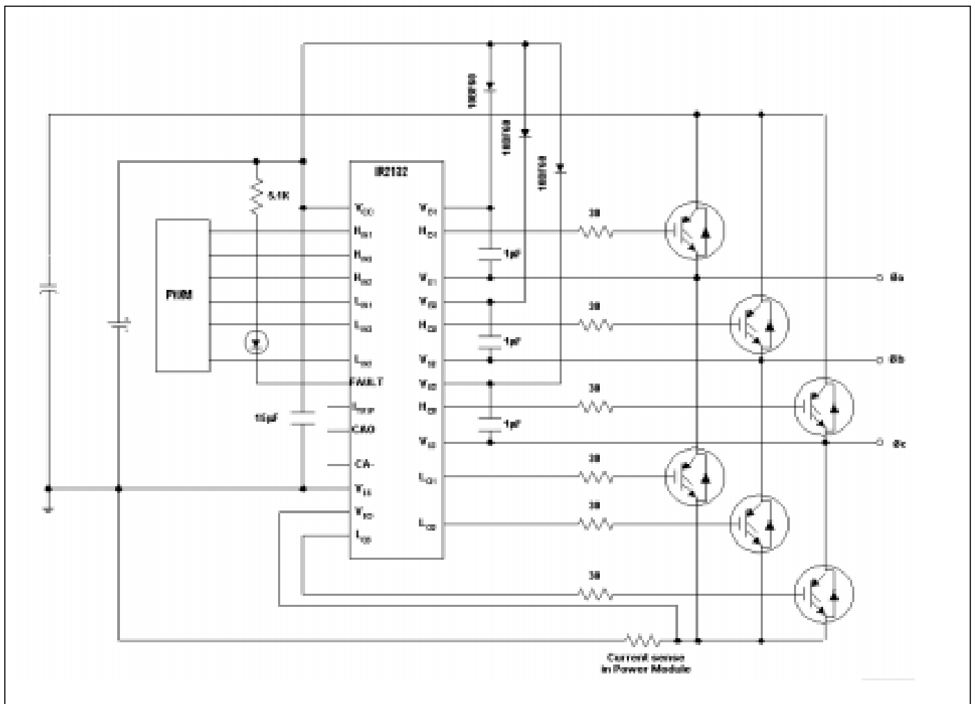
Figure 10. Recommended Gate Drive Circuit
