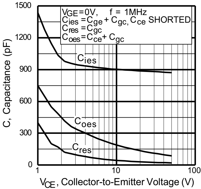
Figure 5a. Typical Capacitance vs Collector-to-Emitter Voltage
