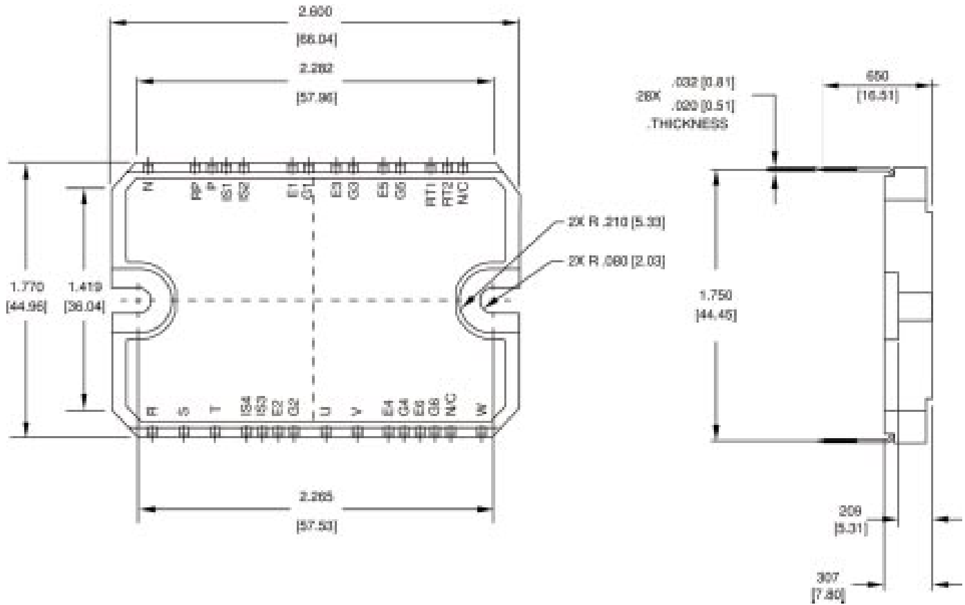
Figure 8a. Package Outline and Mechanical Specifications
