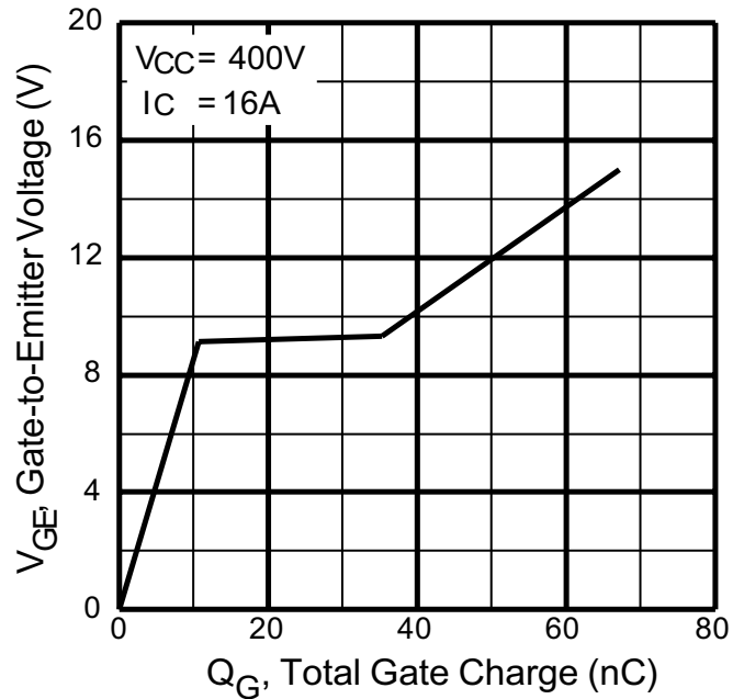
Figure 5b. Typical Gate Charge vs Gate-to-Emitter Voltage
