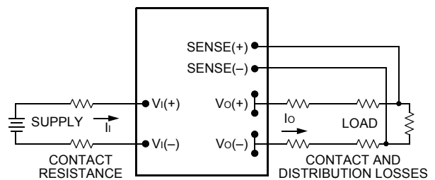
Figure 23. Effective Circuit Configuration for Single-Module Remote-Sense Operation
