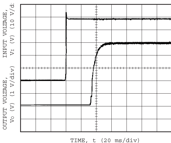
Figure 17. Typical JAHW100A Startup at applied V_{IN}
