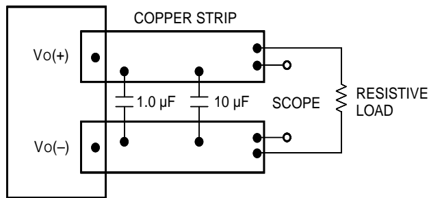
Figure 13. Input Reflected-Ripple Test Setup
