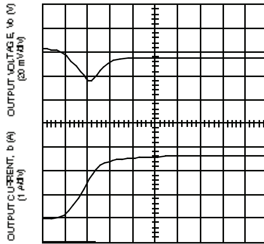
TIME, t (100 μs/div)
