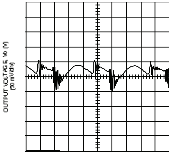
TIME, t (500 ns/div)
