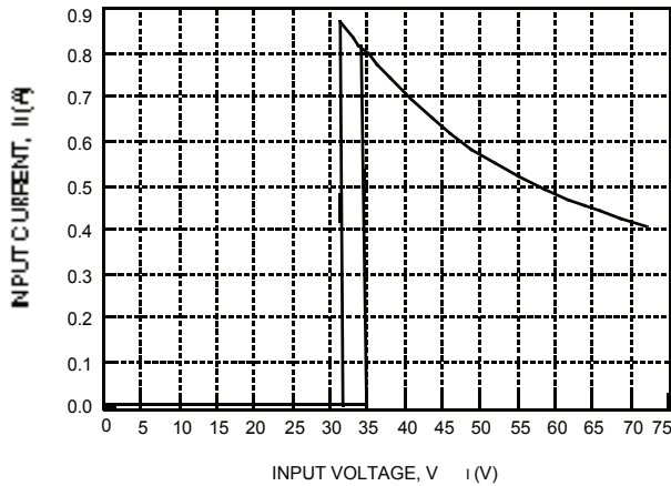
Figure 1. Typical JW050D Input Characteristics at Room Temperature
