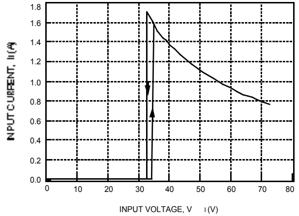
Figure 3. Typical JW100D Input Characteristics at Room Temperature
