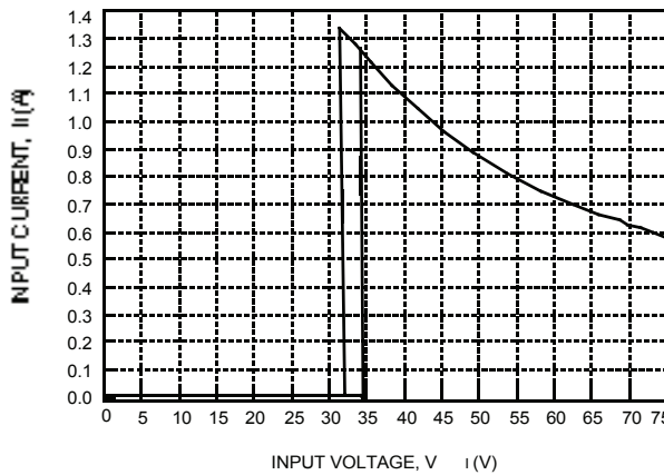
Figure 2. Typical JW075D Input Characteristics at Room Temperature
