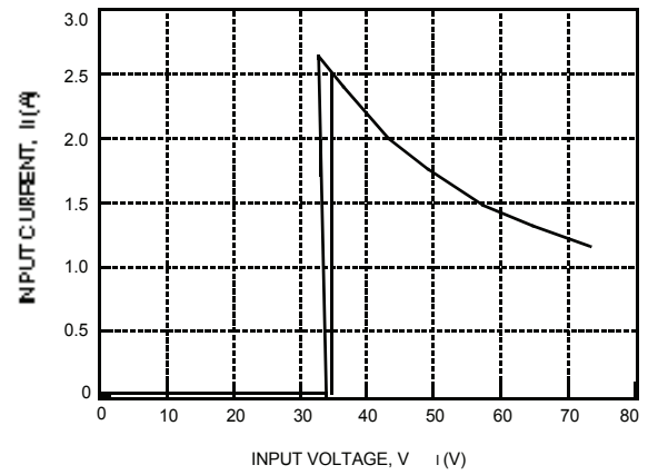
Figure 4. Typical JW150D Input Characteristics at Room Temperature
