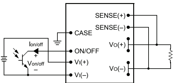
Figure 11. Remote On/Off Implementation
