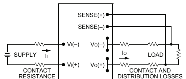
Figure 12. Effective Circuit Configuration for Single-Module Remote-Sense Operation
