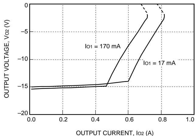
Figure 15. MW005CL Typical Output Characteristics ( V_{O2} vs. I_{O2} ) with V_I = 48 V and T_A = 25 °C
