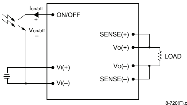
Figure 22. Remote On/Off Implementation
