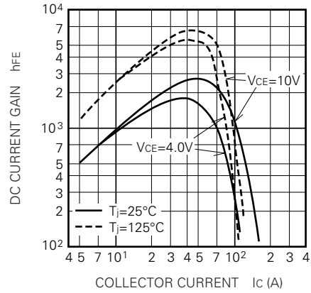
DC CURRENT GAIN VS. COLLECTOR CURRENT (TYPICAL)
