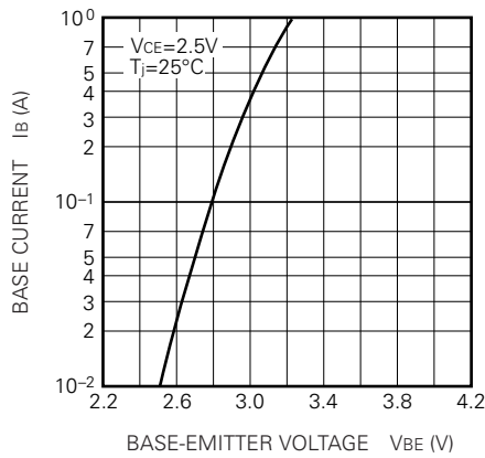
COMMON EMITTER INPUT CHARACTERISTIC (TYPICAL)
