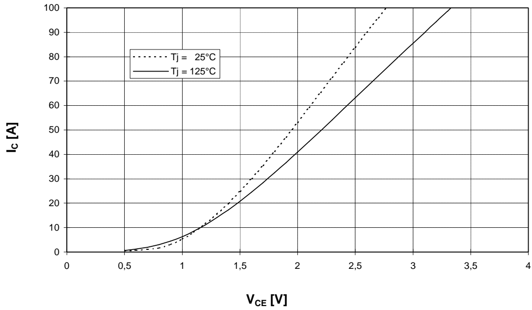
Output characteristic brake-chopper-IGBT (typical)
