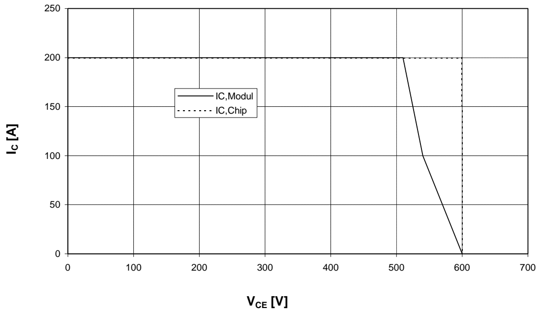
Sicherer Arbeitsbereich Wechselr. (RBSOA) I_C = f(V_{CE}) Reverse bias safe operating area Inverter (RBSOA) T_{vi} = 125^\circ\text{C}, V_{GE} = \pm 15\text{V}, R_G = 15 \text{ Ohm}
