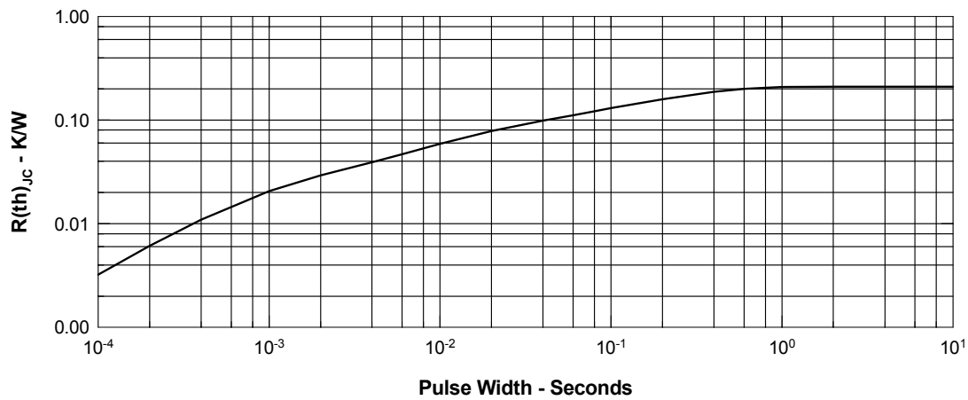
Figure 10. Transient Thermal Resistance
