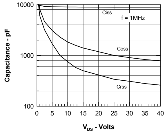
Figure 8. Capacitance Curves
