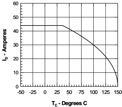
Figure 5. Drain Current vs. Case Temperature
