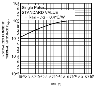
TRANSIENT THERMAL IMPEDANCE CHARACTERISTICS (IGBT per 1 element)
