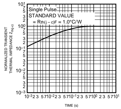
TRANSIENT THERMAL IMPEDANCE CHARACTERISTICS (FWDi per 1 element)
