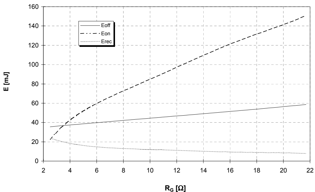
Schaltverluste (typisch) E_{on} = f(R_G) , E_{off} = f(R_G) , E_{rec} = f(R_G) Switching losses (typical) V_{GE} = \pm 15V , I_c = 300A , V_{CE} = 600V , T_{vj} = 125^\circ C
