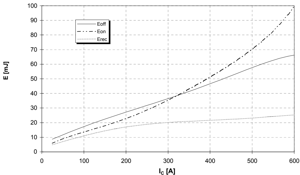
Schaltverluste (typisch) E_{on} = f(I_c) , E_{off} = f(I_c) , E_{rec} = f(I_c) Switching losses (typical) V_{GE} = \pm 15V , R_G = 3,3 \Omega , V_{CE} = 600V , T_{vj} = 125^\circ C
