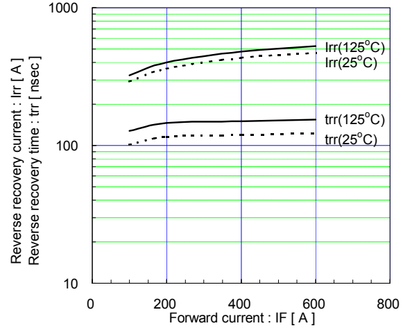
Reverse recovery characteristics (typ.) V_{CC}=600\text{V} , V_{GE}=\pm 15\text{V} , R_G=1.5\Omega
