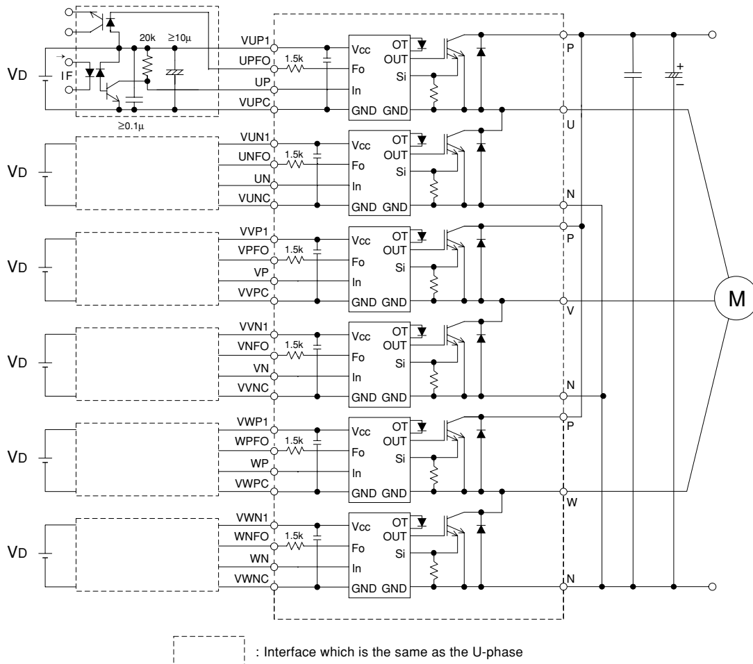
Fig. 8 Application Example Circuit
