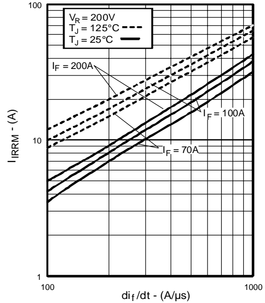
Fig. 6 - Typical Recovery Current vs. di_f/dt , (per Leg)
