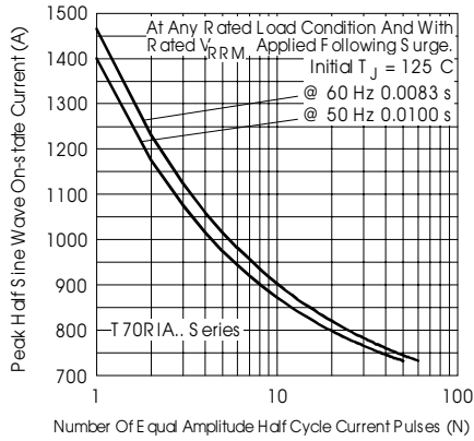
Fig. 16 - Maximum Non-Repetitive Surge Current
