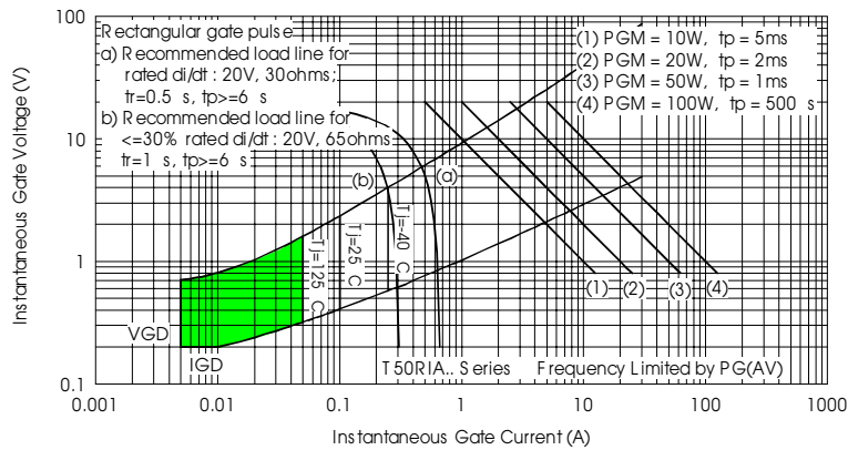
Fig. 9 - Gate Characteristics
