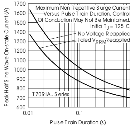
Fig. 17 - Maximum Non-Repetitive Surge Current
