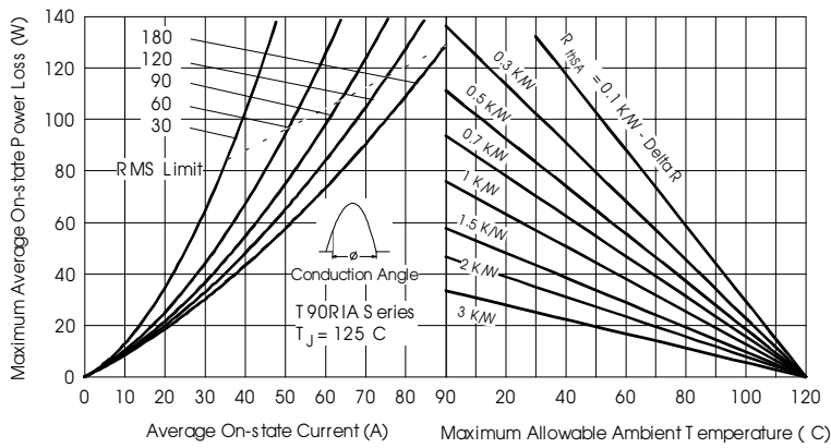
Fig. 29 - On-state Power Loss Characteristics
