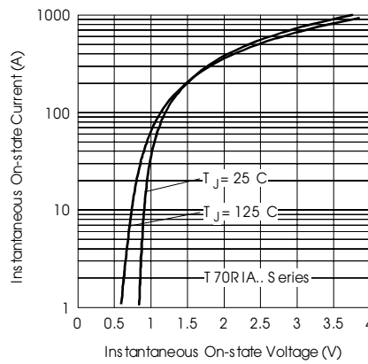
Fig. 10 - On-state Voltage Drop Characteristics
