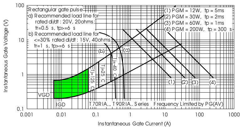
Fig. 19 - Gate Characteristics
