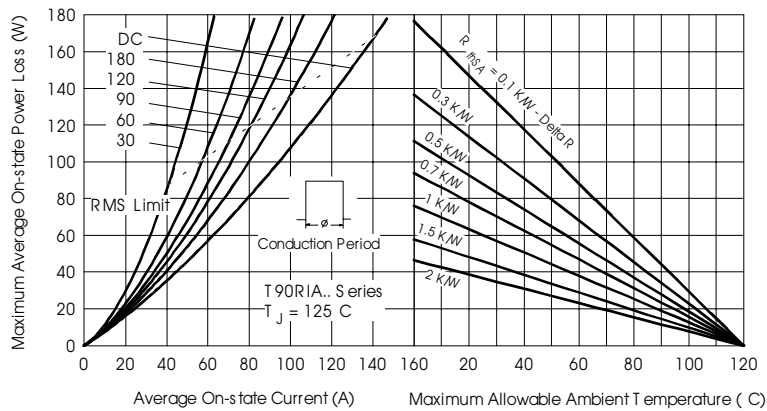
Fig. 29 - On-state Power Loss Characteristics
