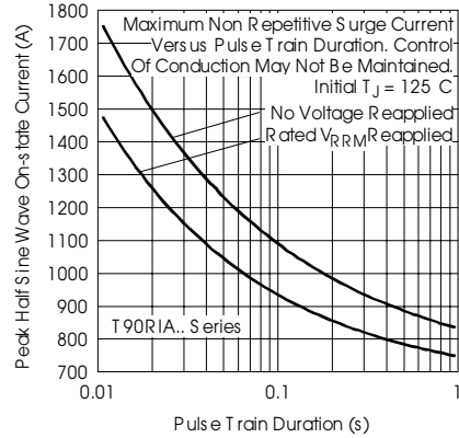
Fig. 28 - Maximum Non-Repetitive Surge Current
