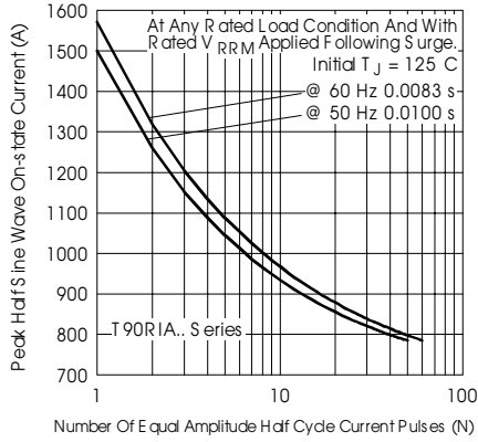
Fig. 27 - Maximum Non-Repetitive Surge Current
