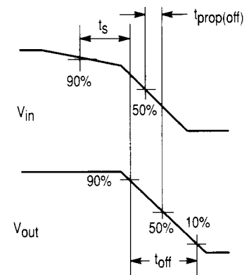
Figure 2. Turn-Off Waveforms
