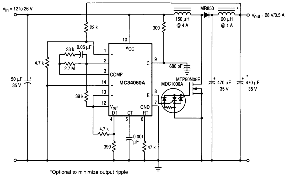
Figure 16. DC-DC Converter
