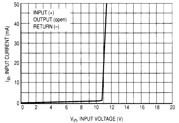
Figure 6. Input Characteristics
