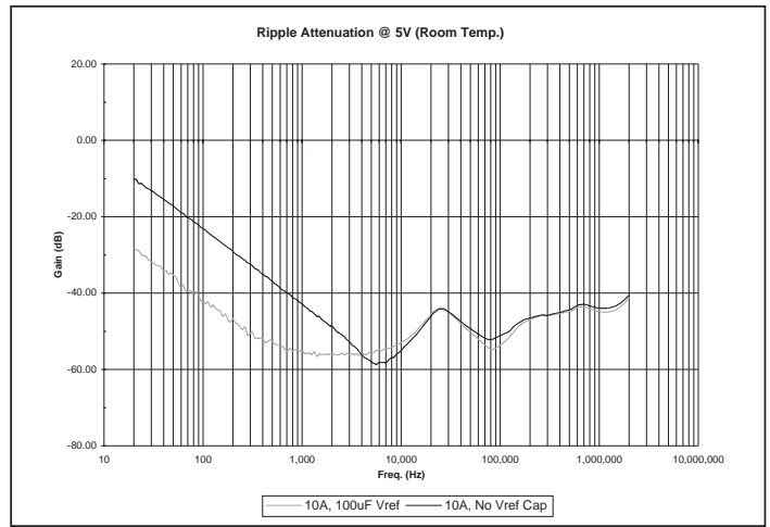
Figure 3a, 3b—Curves demonstrating the small signal attenuation performance as measured on a network analyzer with a typical module at (a) 28V and 10A output and (b) 5V and 10A. The low frequency attenuation can be enhanced by connecting a 100μF capacitor, CHR, to the VREF pin as shown in Figures 1 and 2.
