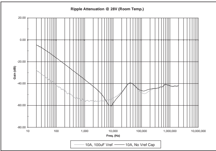
Figure 3a, 3b—Curves demonstrating the small signal attenuation performance as measured on a network analyzer with a typical module at (a) 28V and 10A output and (b) 5V and 10A. The low frequency attenuation can be enhanced by connecting a 100μF capacitor, CHR, to the VREF pin as shown in Figures 1 and 2.
