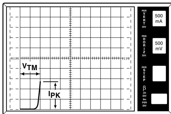
Figure AN1006.25 V_{TM(Forward)} = 950 mV at I_{PK} = 1.4 A
