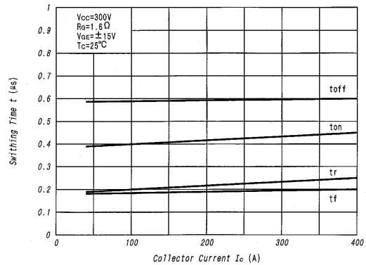
Fig. 6 Collector Current vs. Switching Time (Typical)
