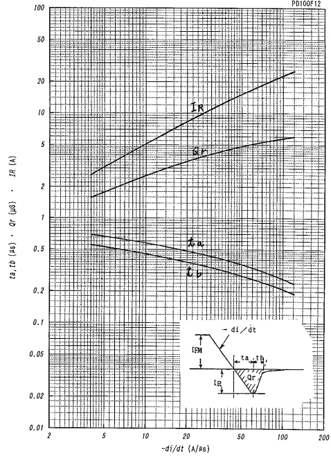
逆回復特性(代表例) REVERSE RECOVERY CHARACTERISTICS (TYP)
