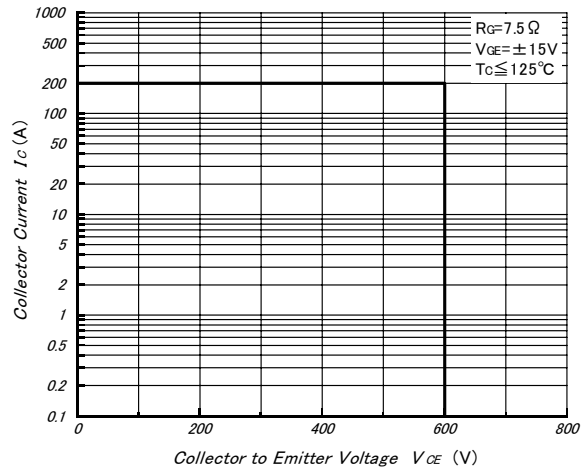
Fig.10- Reverse Bias Safe Operating Area (Typical)
