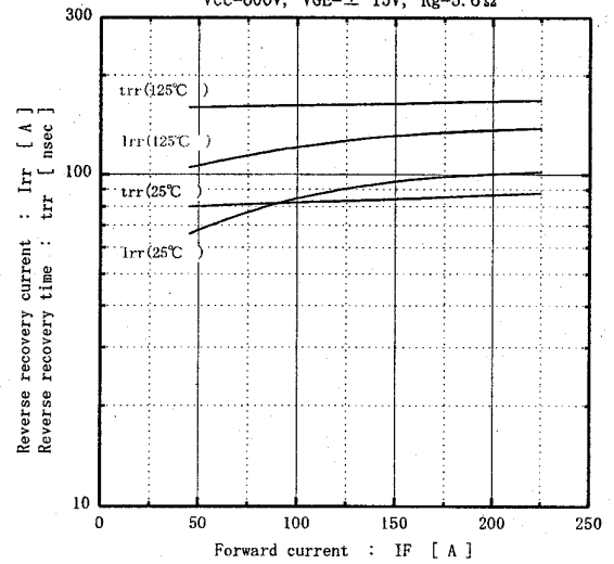
Reverse recovery characteristics (typ.) Vcc=600V, VGE=± 15V, Rg=5.6Ω
