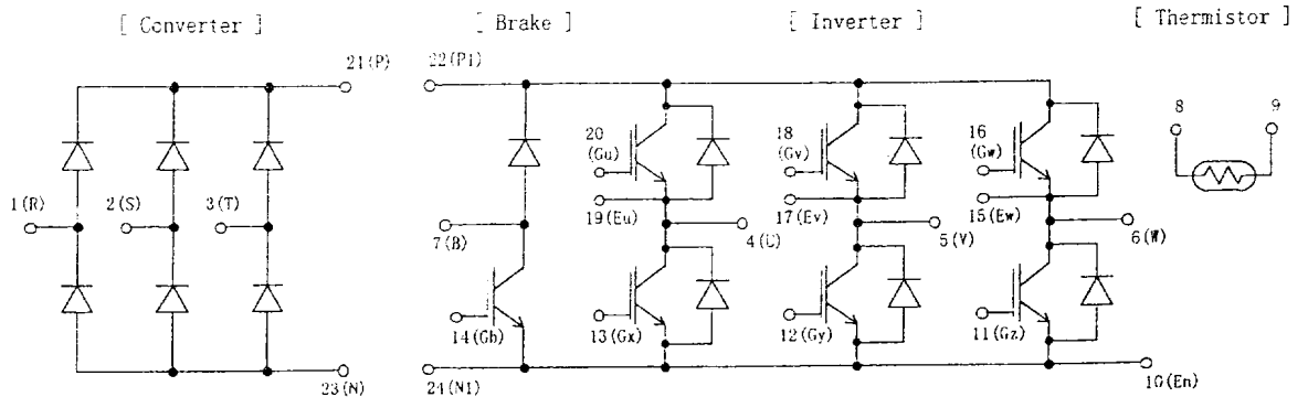
2. Equivalent circuit
