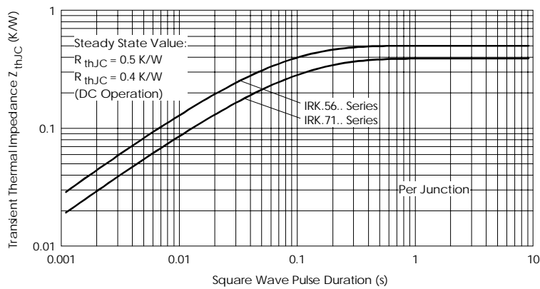
Fig. 21 - Thermal Impedance Z_{thJC} Characteristic
