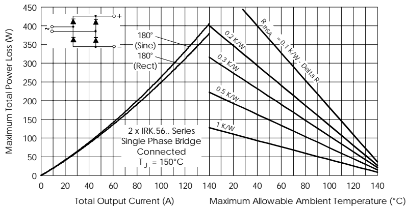
Fig. 8 - Forward Power Loss Characteristics
