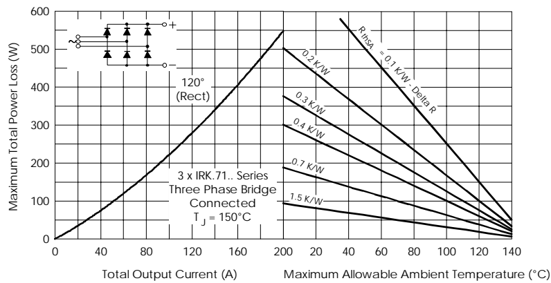
Fig. 18 - Forward Power Loss Characteristics
