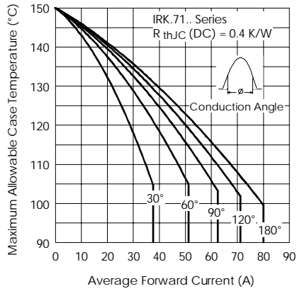
Fig. 10 - Current Ratings Characteristics
