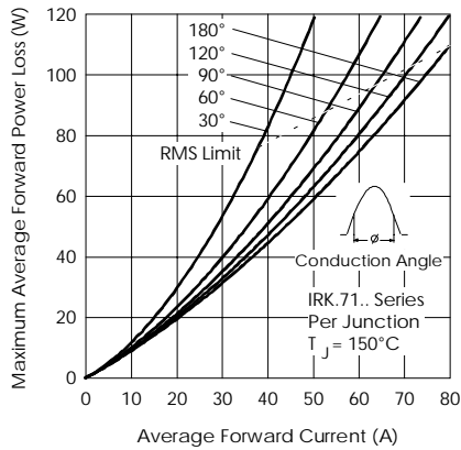
Fig. 12 - Forward Power Loss Characteristics
