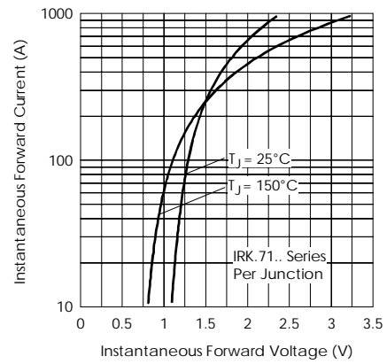
Fig. 20 - Forward Voltage Drop Characteristics
