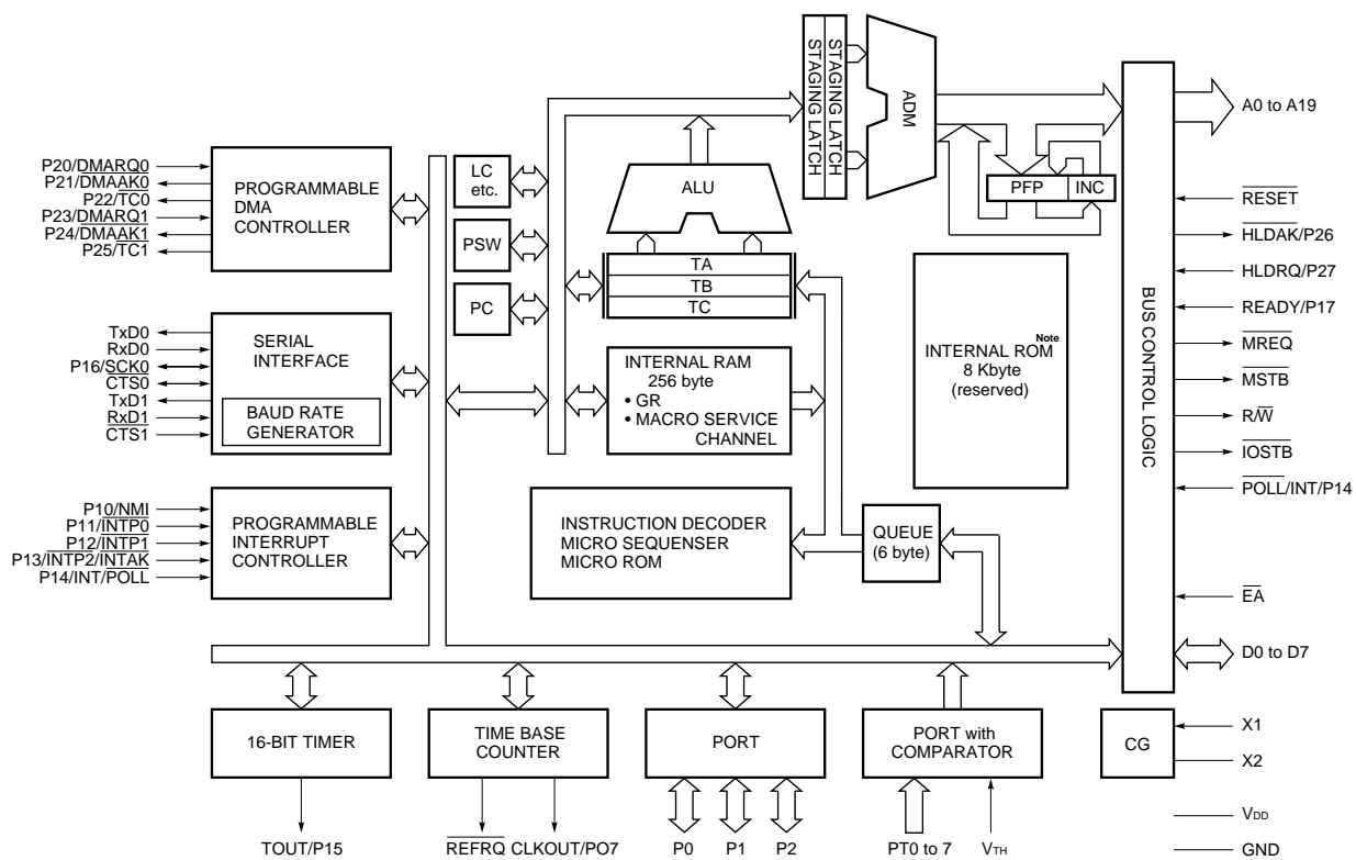
INTERNAL BLOCK DIAGRAM
