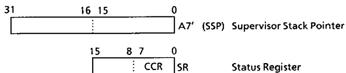
Figure 1.2 Supervisor Programming Model Supplement
