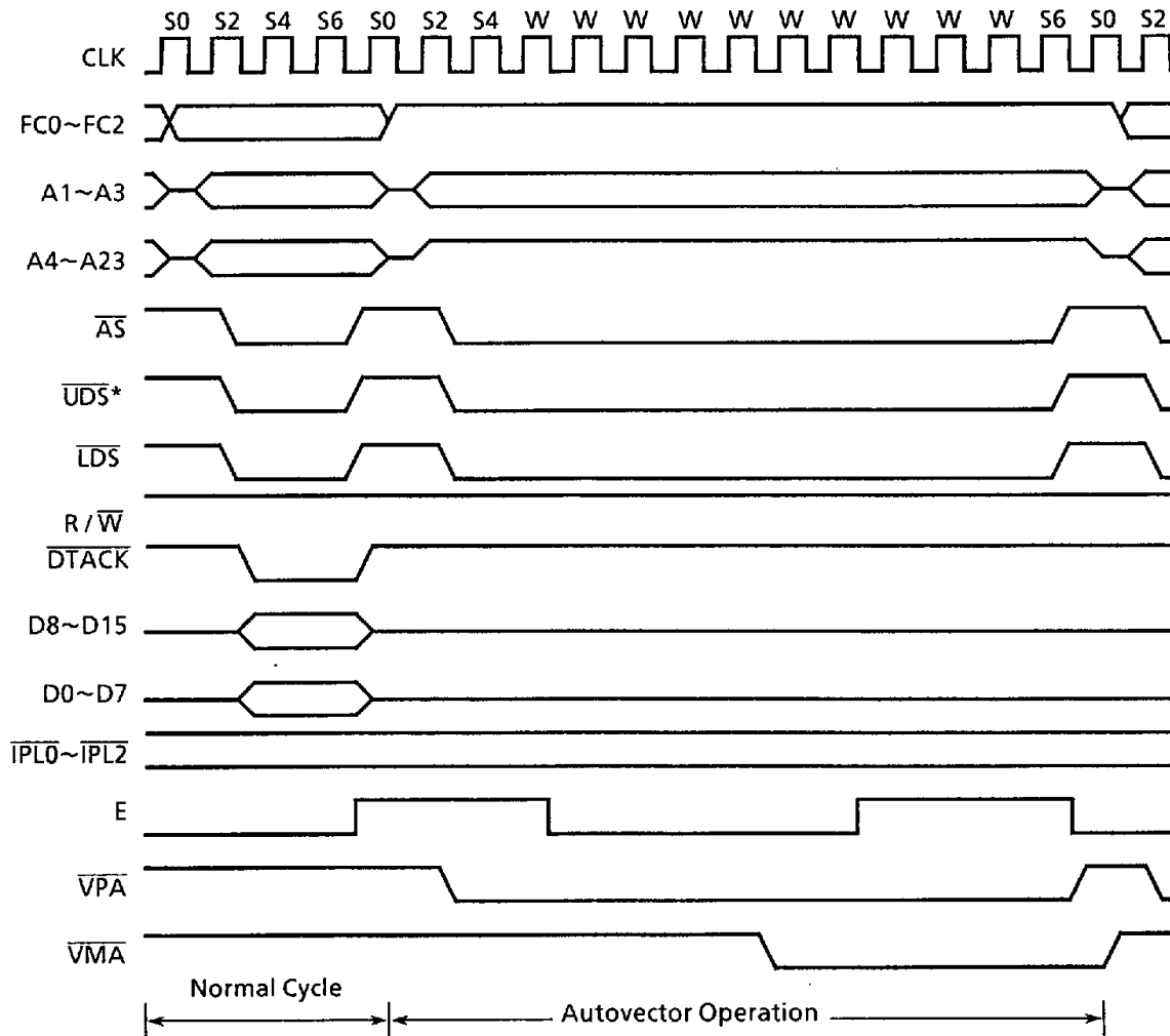
Figure 6.4 Autovector Operation Timing Diagram
