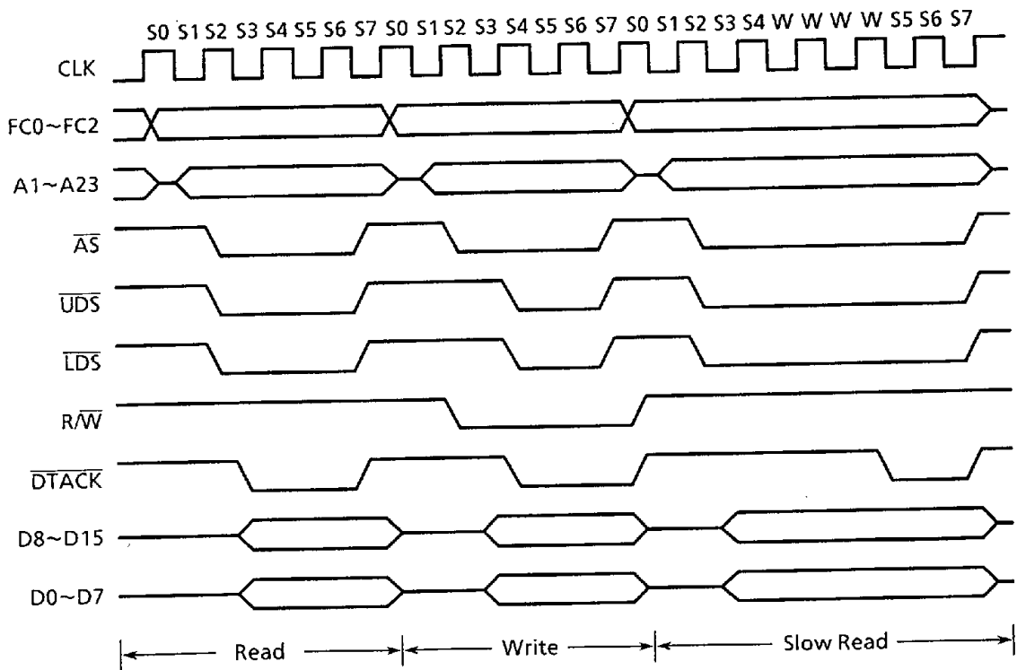
Figure 4.4 Read and Write Cycle Timing Diagram
