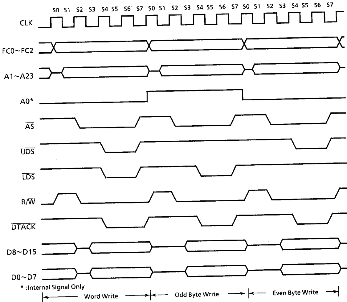
Figure 4.8 Word and Byte Write Cycle Timing Diagram
