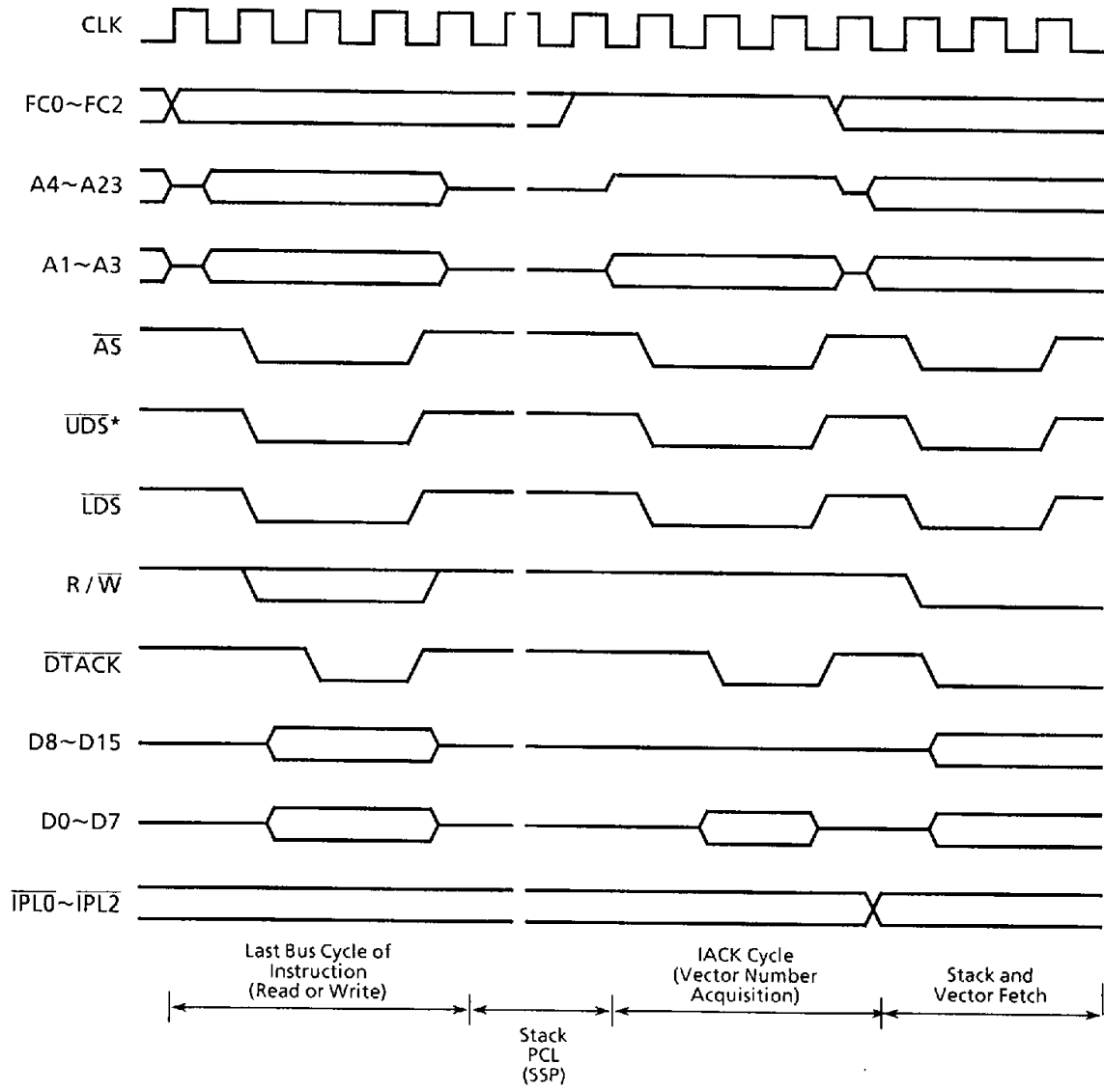
Figure5.6 Interrupt Acknowledge Cycle Timing Diagram
