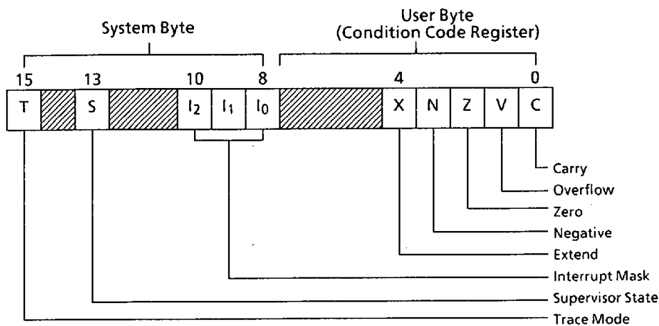
Figure 1.3 Status Register
