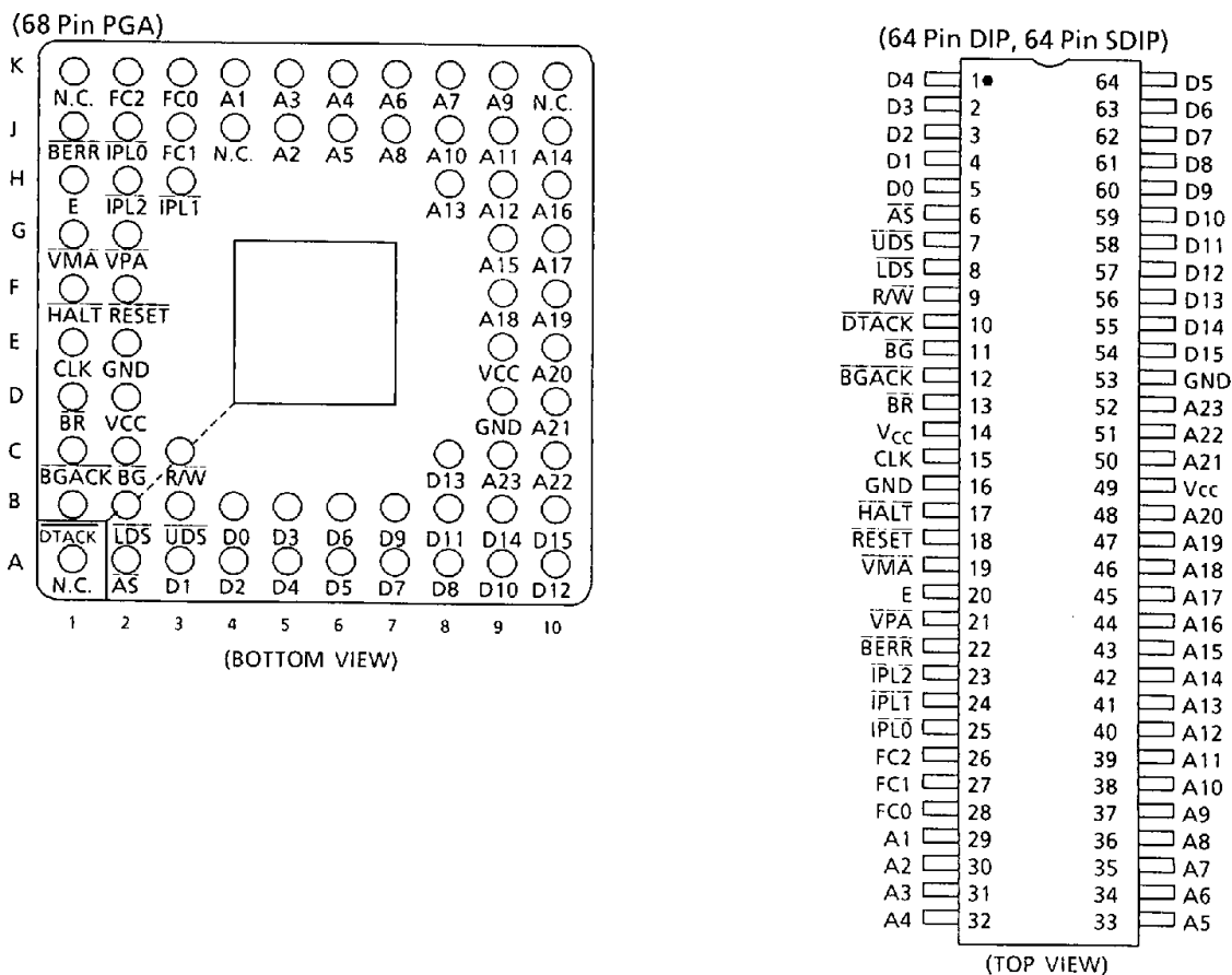
Figure 4.1 Input and Output Signals Pin Assignments (1/2)
