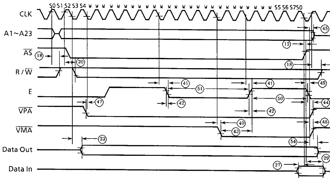
Figure 8.5 TMP68HC000 to 6800 Peripheral Timing Diagram – Best Case
