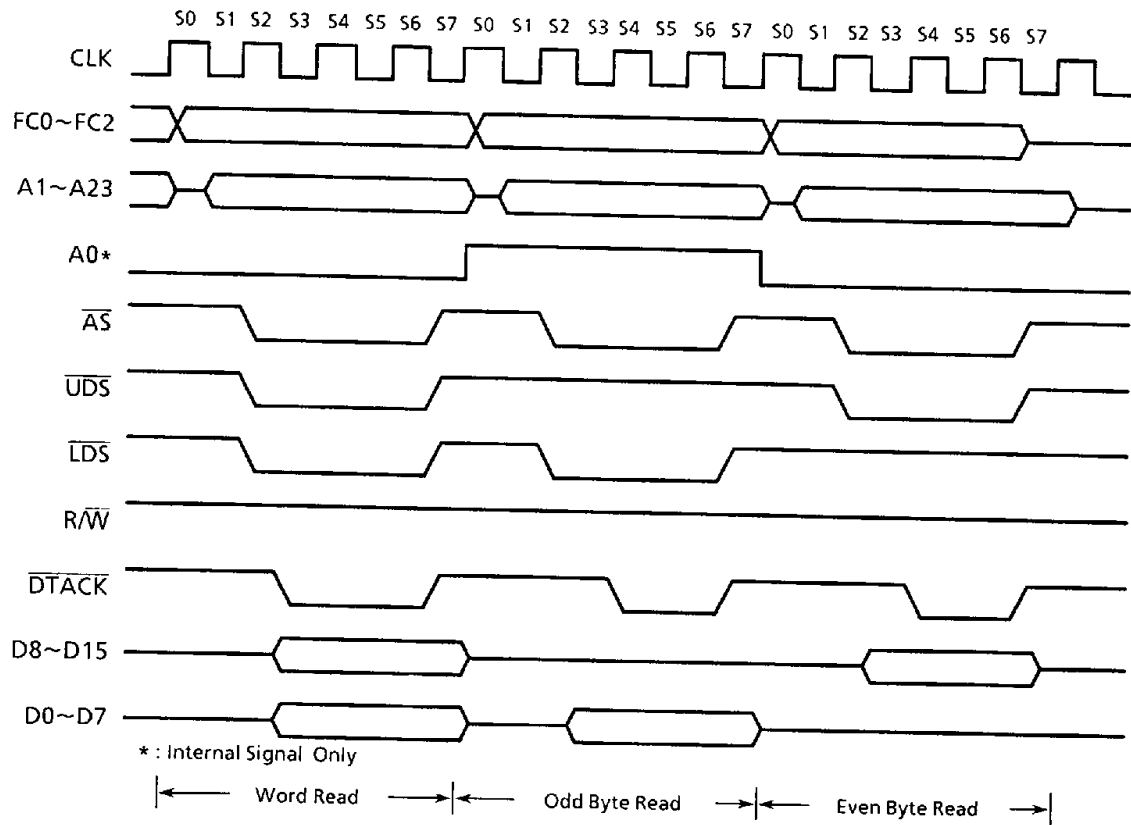
Figure 4.5 Word and Byte Read Cycle Timing Diagram
