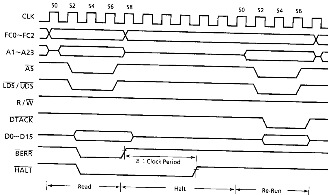
Figure 4.19 Re-Run Bus Cycle Timing Diagram
