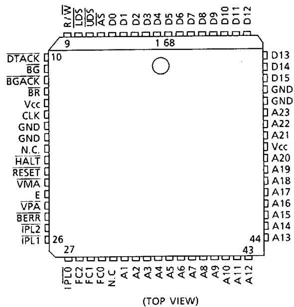
4.1 Input and Output Signals Pin Assignments (2/2)
