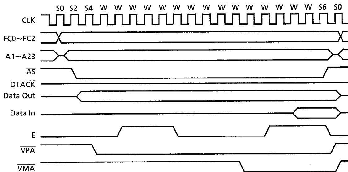
Figure 6.3 TMP68HC000 to 6800 Peripheral Timing – Worst Case
