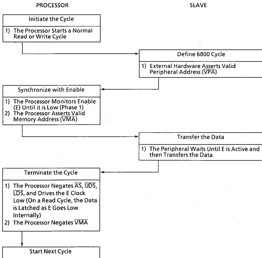
Figure 6.1 6800 Interfacing Flowchart
