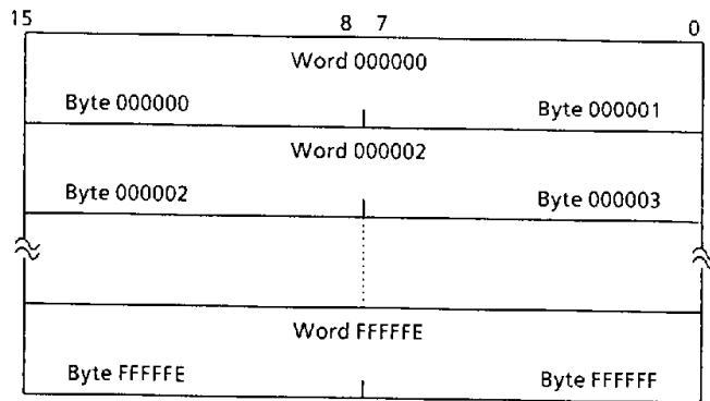
Figure 2.1 Word Organization in Memory
