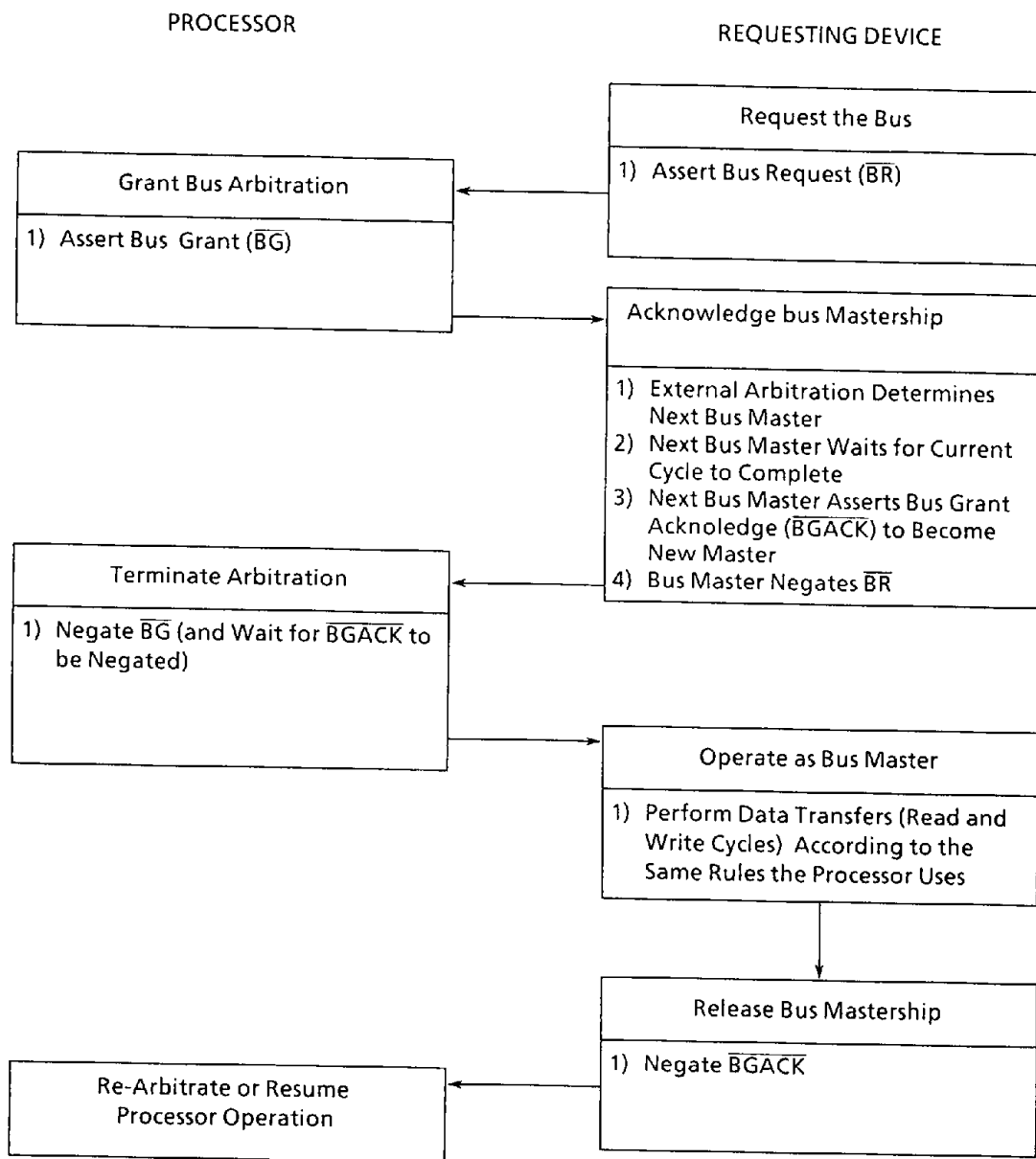
Figure 4.11 Bus Arbitration Cycle Flowchart
