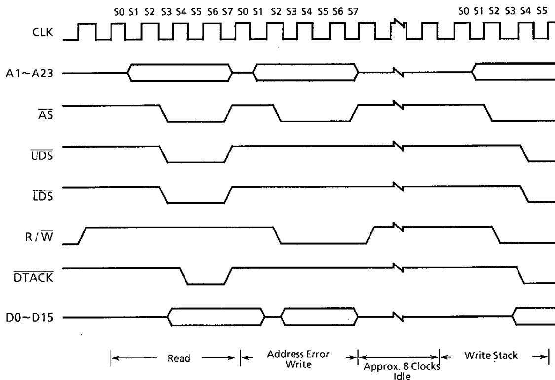
Figure 5.9 Address Error Timing Diagram
