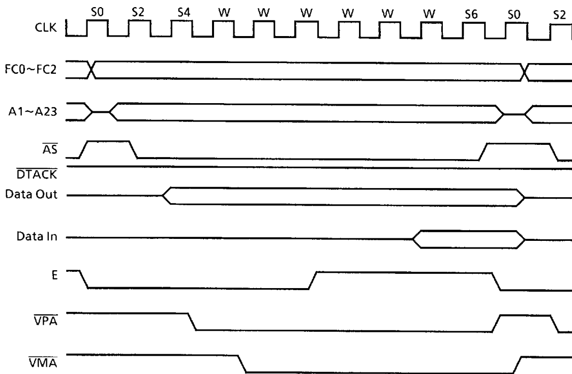
Figure 6.2 TMP68HC000 to 6800 Peripheral Timing – Best Case
