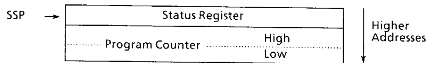
Figure 5.4 Exception Stack Order (Groups 1 and 2)
