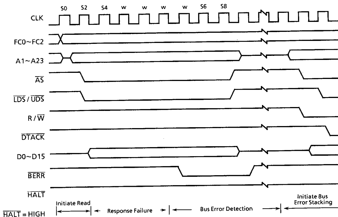
Figure 4.18 Bus Error Timing Diagram
