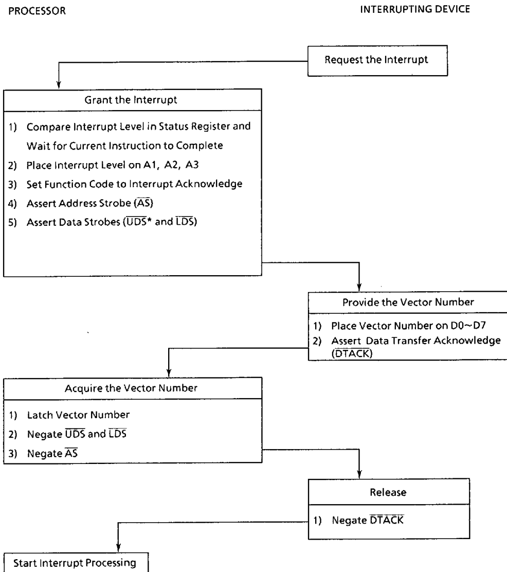
Figure5.5 Vector Acquisition Flowchart
