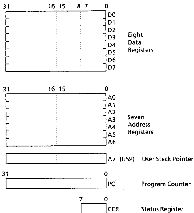
Figure 1.1 User Programming Model
