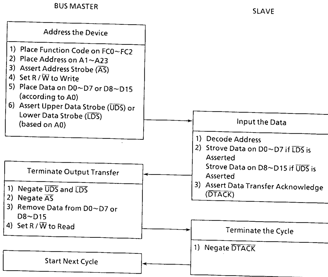
Figure 4.7 Byte Write Cycle Flowchart
