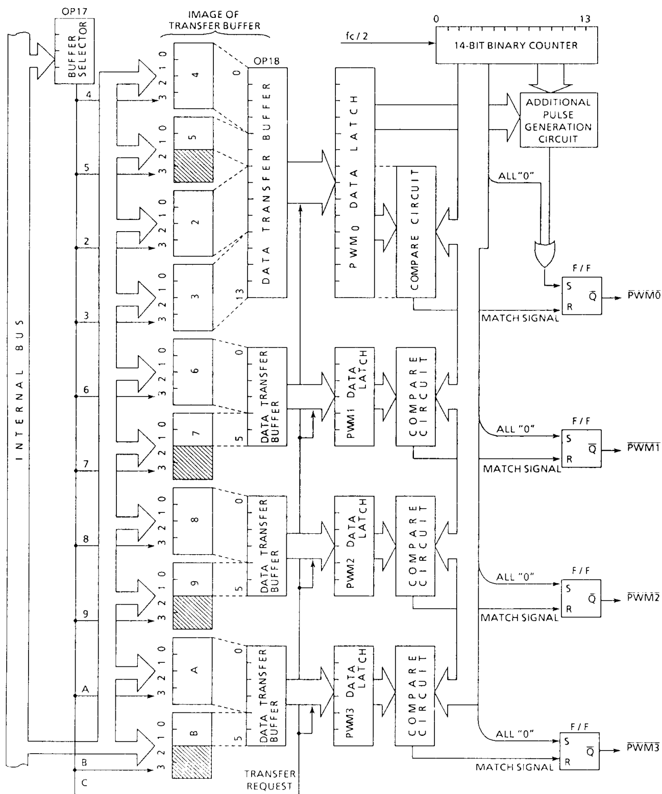
Figure 2-7. Pulse Width Modulation Circuit
