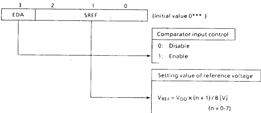
Figure 2-5. Control Command Register
