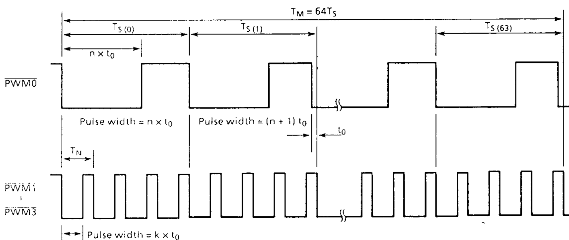
Figure2-6. \overline{\text{PWM}} Output Waveform (It is shown to the additional pulse T_S(1) and T_S(63) of the \overline{\text{PWM0}} )
