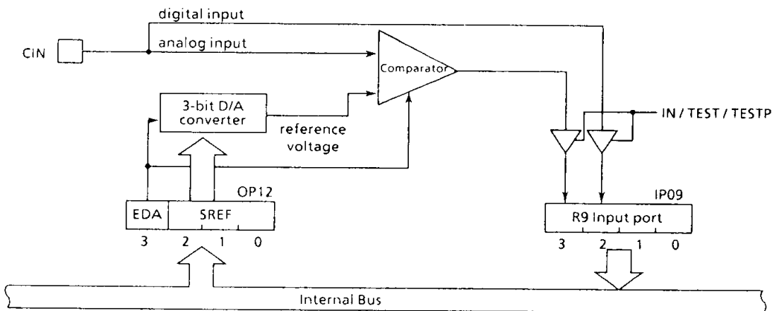
Figure 2-4. Comparator input Circuit
