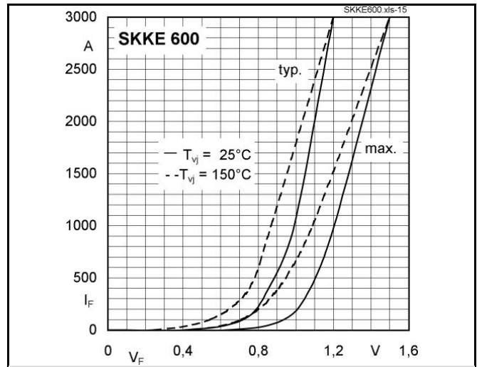
Fig. 15 Forward characteristics
