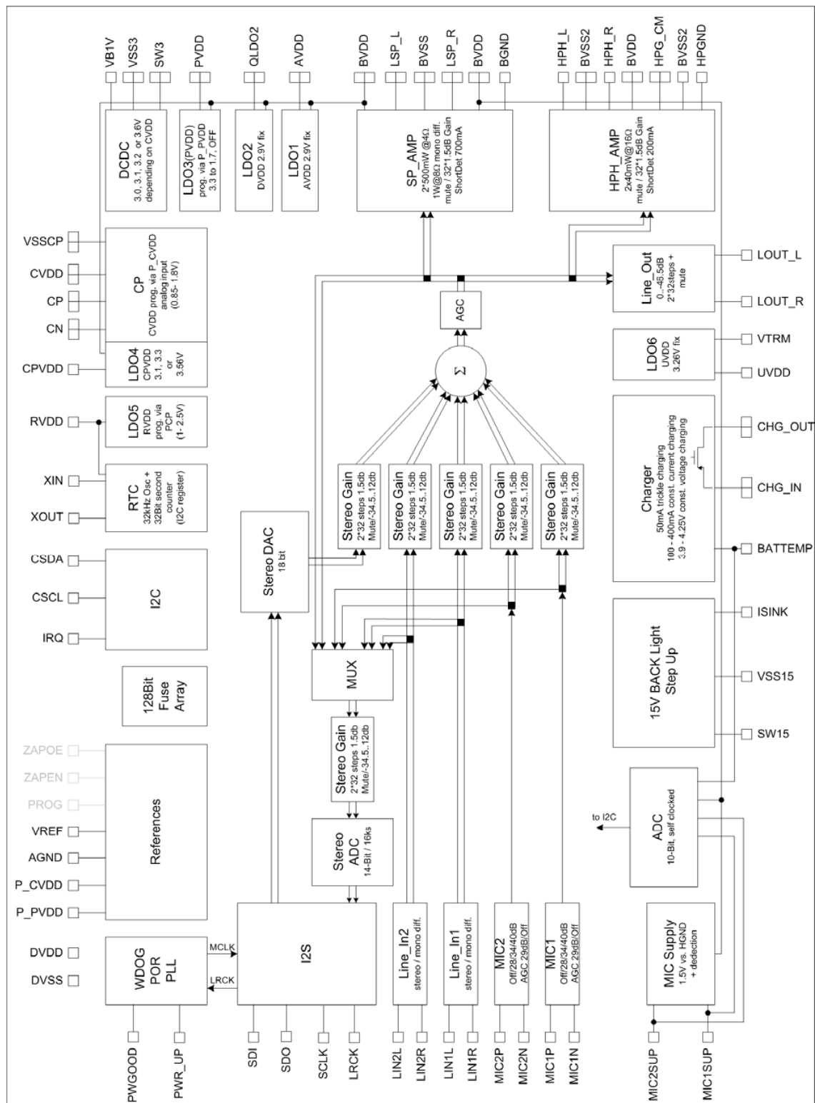
Figure 1 AS3515 Block Diagram
