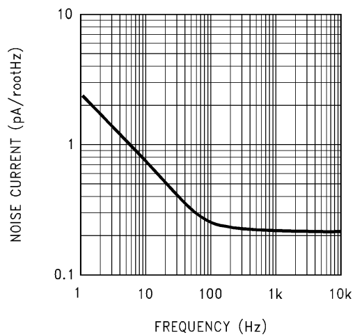
Noise Current vs. Frequency
