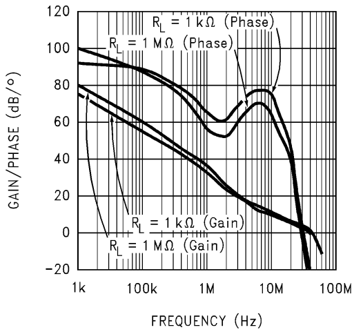
Open Loop Gain/Phase ( V_S = 24V )
