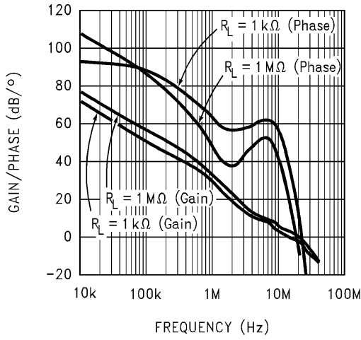
Open Loop Gain/Phase ( V_S = 5V )
