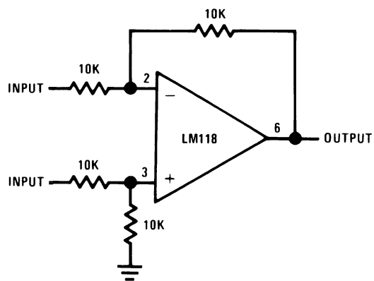
Differential Amplifier
