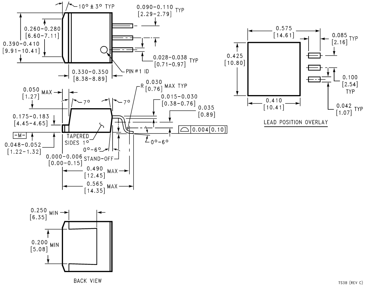
TO-263 3-Lead Plastic Surface Mount Package
