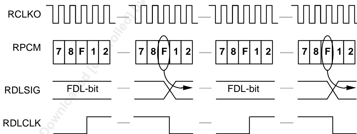
Figure 19 - ESF 4Kbit/s Receive Datalink Interface
