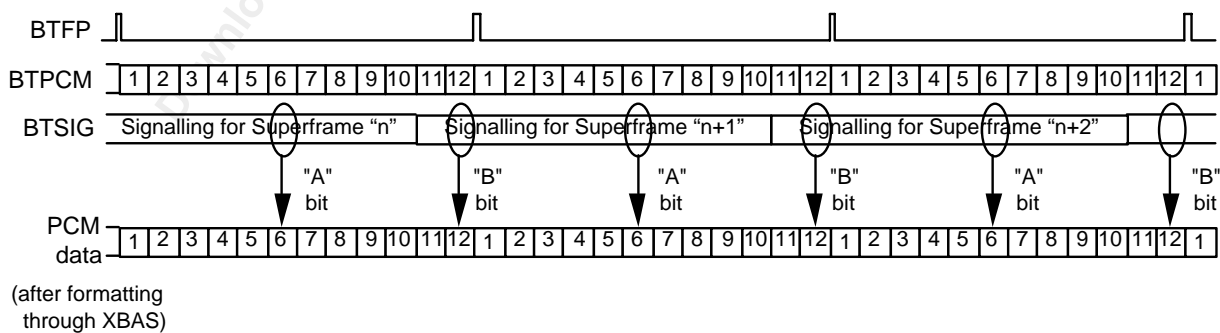
Figure 30 - 1.544MHz Transmit Backplane Interface - without signalling alignment
