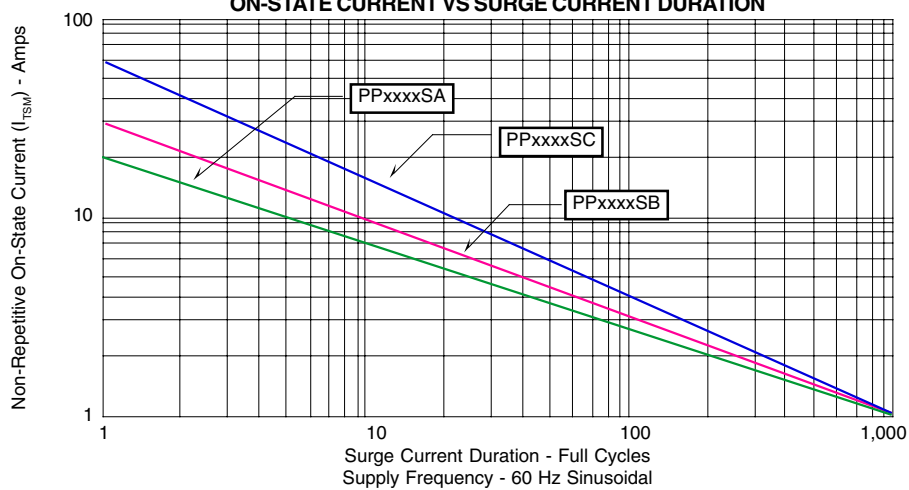
FIGURE 3 ON-STATE CURRENT VS SURGE CURRENT DURATION
