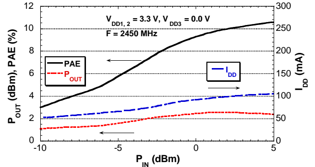
Output Power, and Drain Current vs. Input Power for Low Current "Bypass" Mode ( V_{DD1,2} = 3.3 V, V_{DD3} = 0.0 V)
