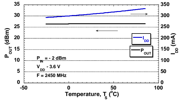
Output Power and Drain Current vs. Temperature at V_{DD} = +3.6\text{ V}
