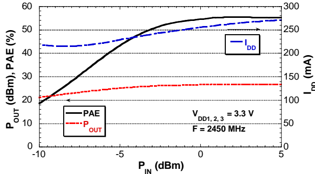
Output Power, Drain Current and Efficiency vs. Input Power
