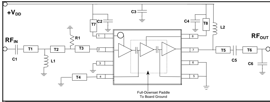
Figure 12 Evaluation Board Schematic
