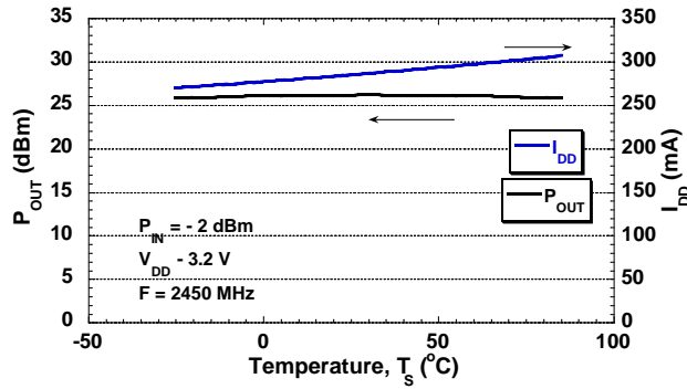
Output Power and Drain Current vs. Temperature at V_{DD} = +3.2\text{ V}
