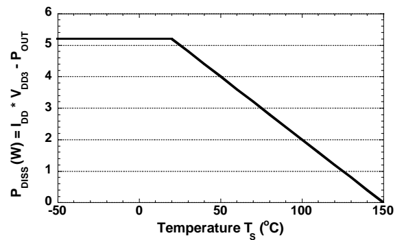
Maximum Operating Temperature ( T_s ) to Maintain <150\text{ }^\circ\text{C} Junction Temperature.
