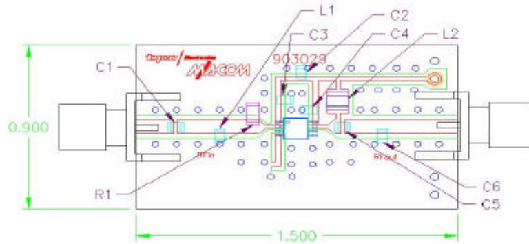
Figure 11 Component layout and printed circuit drawing for evaluation board (60 mil GETEK board).
