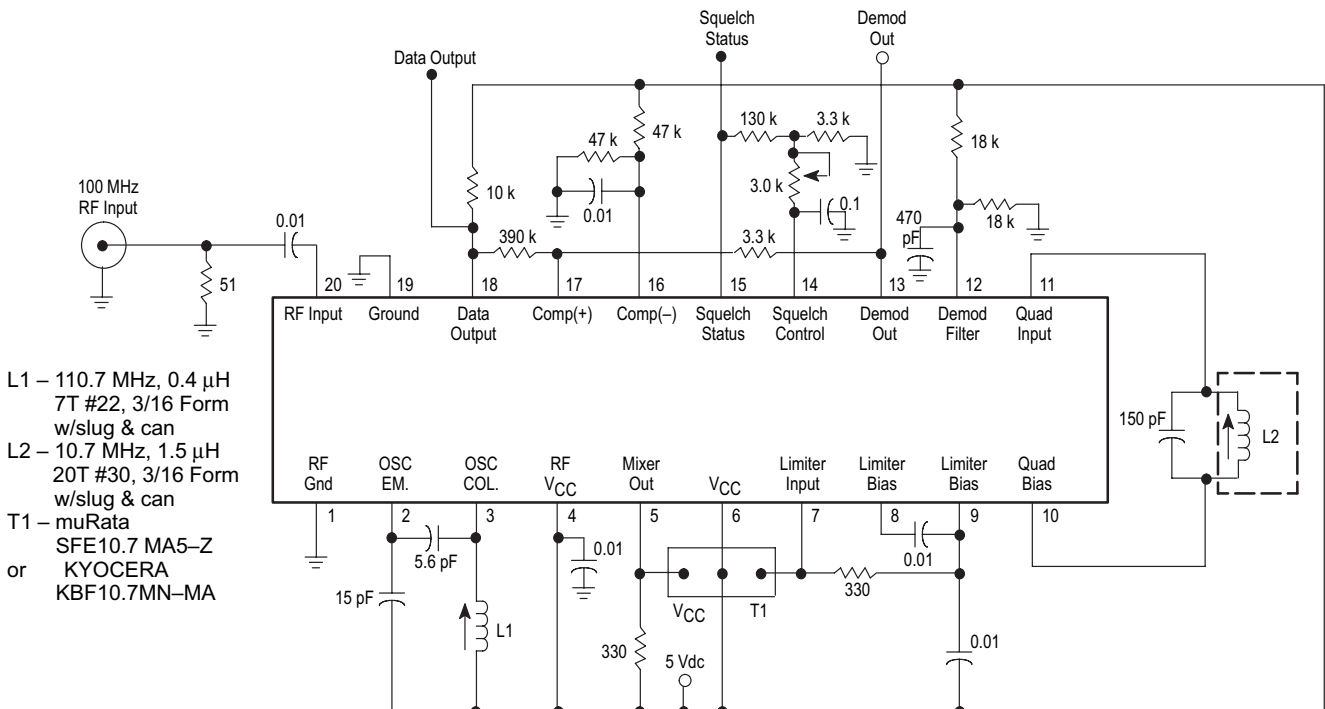
Figure 2. Test Circuit
