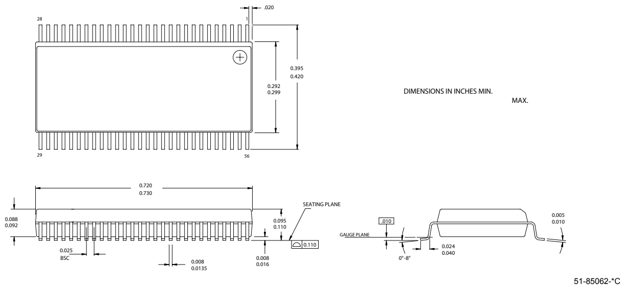
Figure 15-1. 56-lead Shrunken Small Outline Package 056
