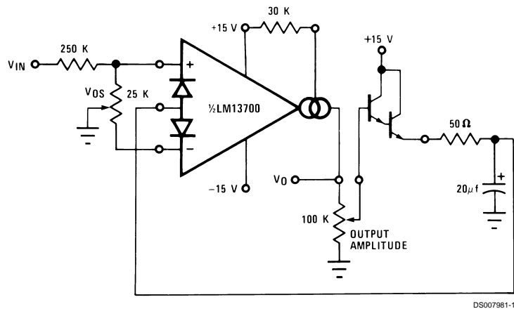
FIGURE 7. AGC Amplifier
