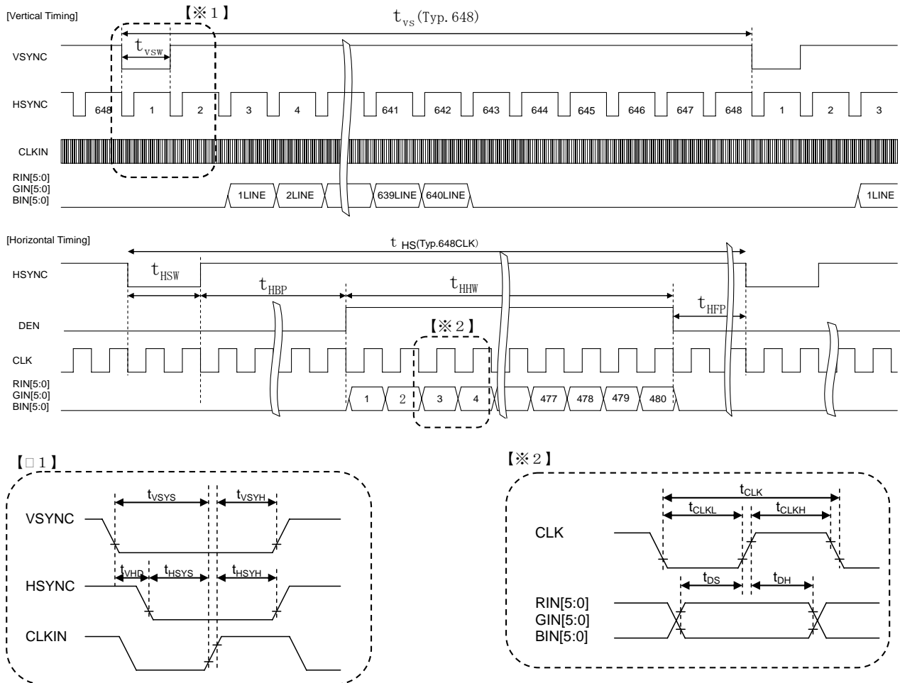
Fig 7-3 LCDIF signal timing in Portrait VGA mode
