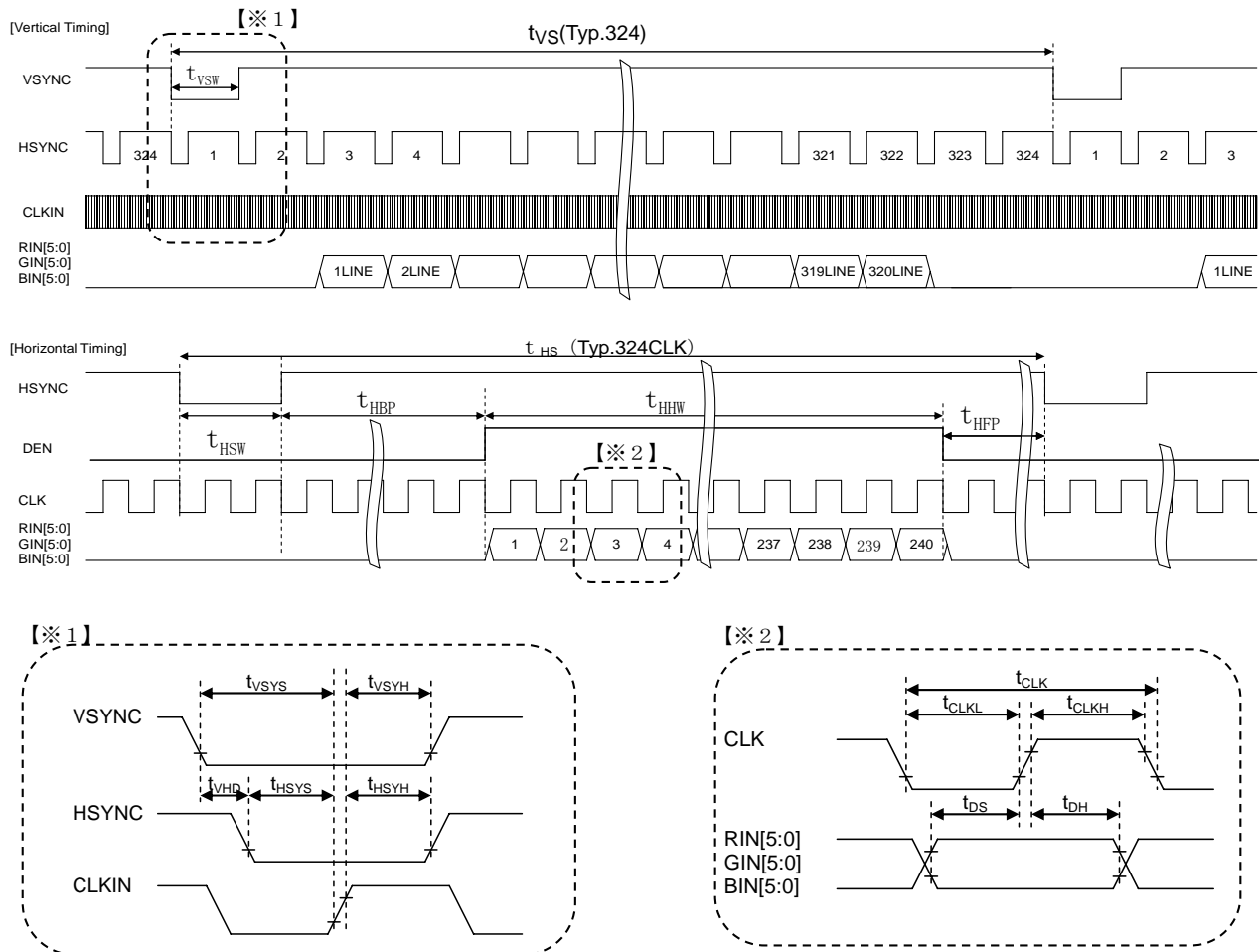
Fig 7-4 LCDIF signal timing in Portrait QVGA mode
