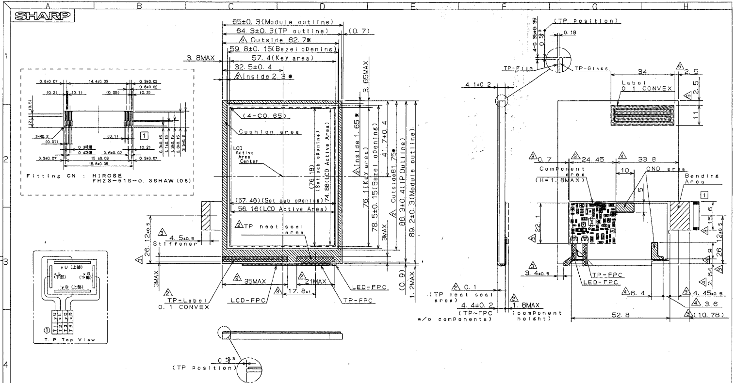
Fig. 1 Outline dimensions
