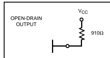
Figure 5. Connection Recommendation for LOCK
