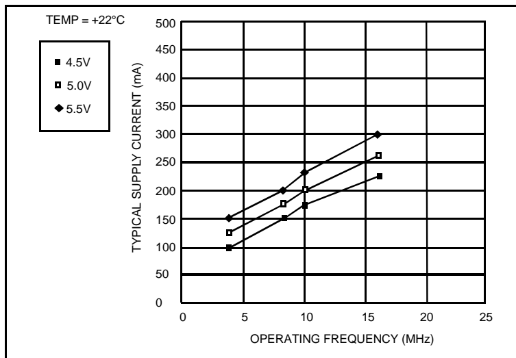
Figure 7. Typical Current vs. Frequency (Room Temp)
