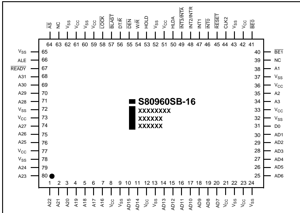
Figure 15. 80-Lead EIAJ Quad Flat Pack (QFP) Package
