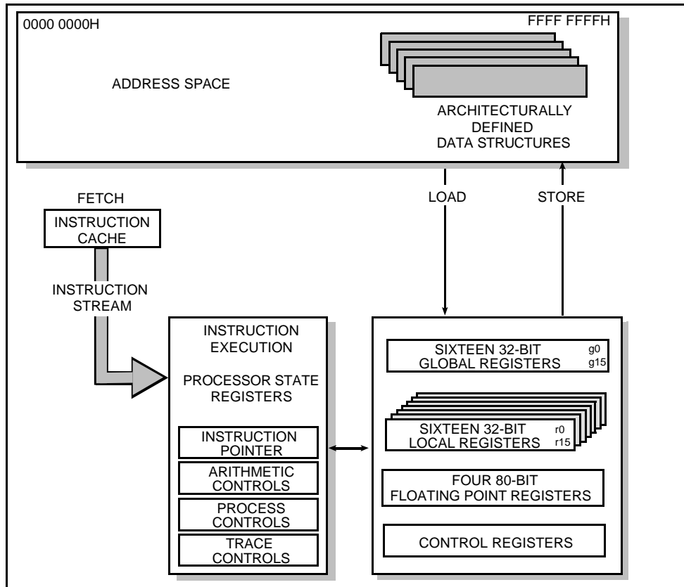
Figure 2. 80960SB Programming Environment
