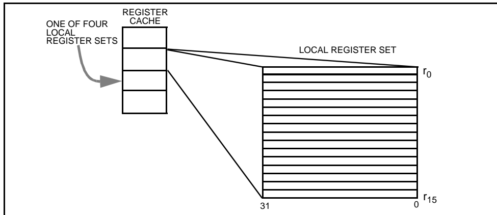
Figure 4. Multiple Register Sets Are Stored On-Chip
