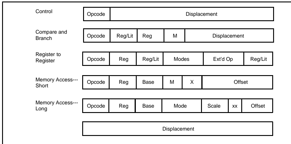
Figure 3. Instruction Formats
