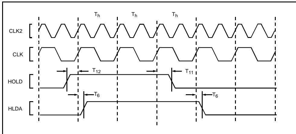
Figure 14. HOLD Timing
