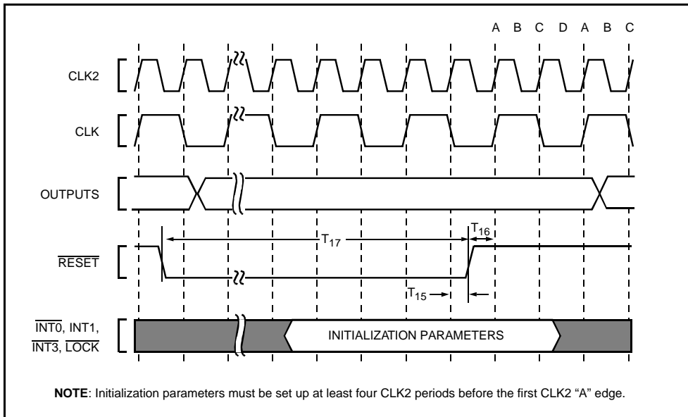
Figure 13. \overline{RESET} Signal Timing
