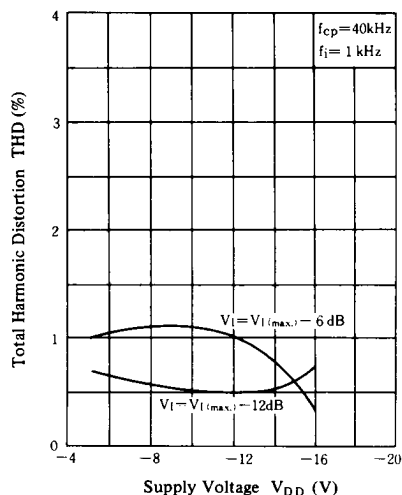
THD - V_{DD}
