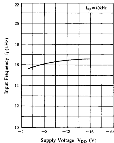
f_i - V_{DD}
