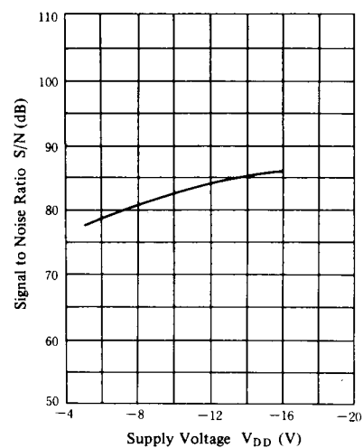
S/N - V_{DD}
