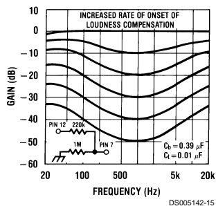
FIGURE 12. Loudness Compensated Volume Characteristic
