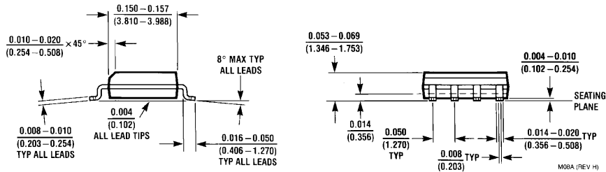
8-Lead (0.150" Wide) Molded Small Outline Package, JEDEC (M) Order Number LM4861 NS Package Number M08A
