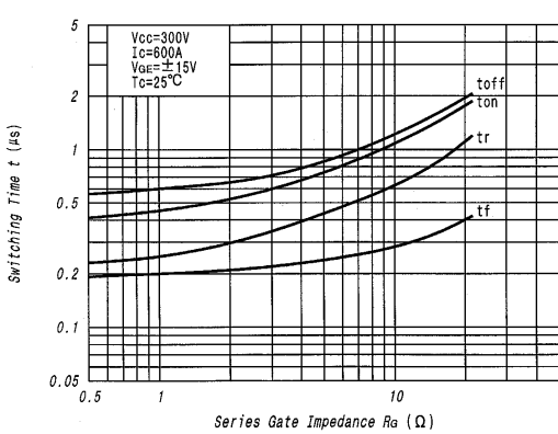
Fig. 7 Series Gate Impedance vs. Switching Time (Typical)
