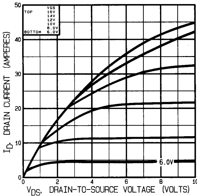
Fig 11. Typical Output Characteristics Post-Irradiation 300K Rads (Si)
