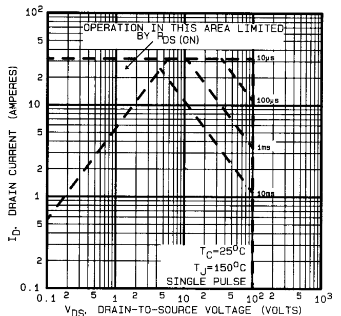
Fig 24. Maximum Safe Operating Area
