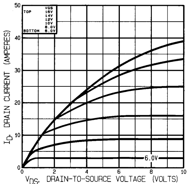
Fig 16. Typical Output Characteristics Post-Irradiation 1 Mega Rads (Si)
