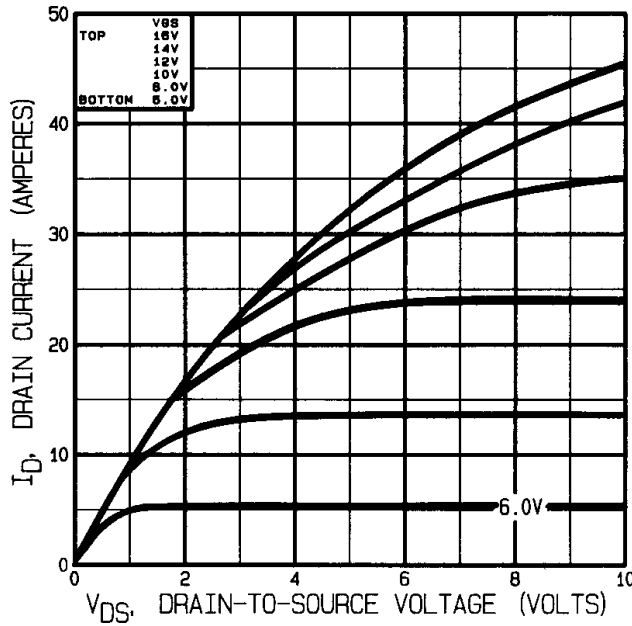
Fig 13. Typical Output Characteristics Pre-Irradiation
