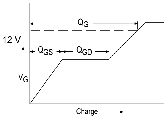
Fig 29a. Basic Gate Charge Waveform
