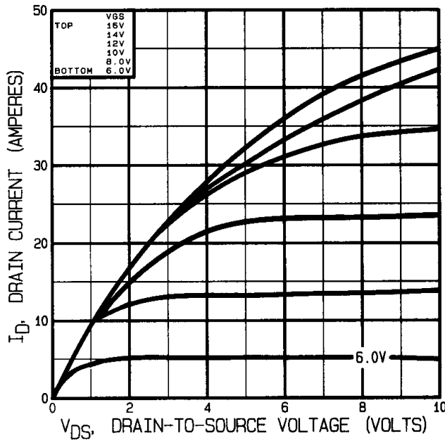
Fig 9. Typical Output Characteristics Pre-Irradiation
