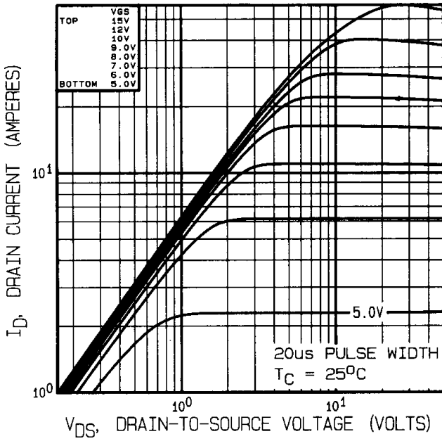
Fig 17. Typical Output Characteristics
