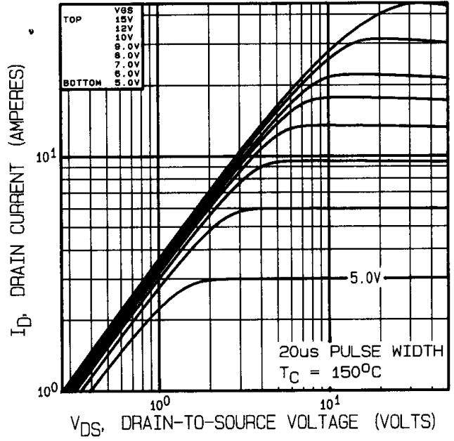
Fig 18. Typical Output Characteristics
