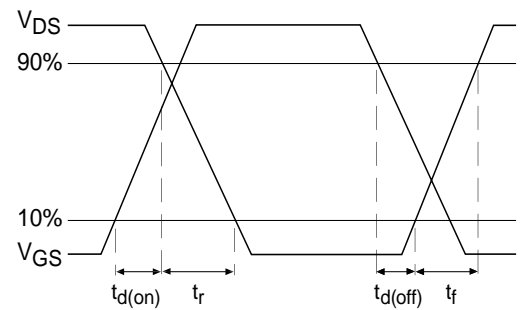
Fig 26b. Switching Time Waveforms
