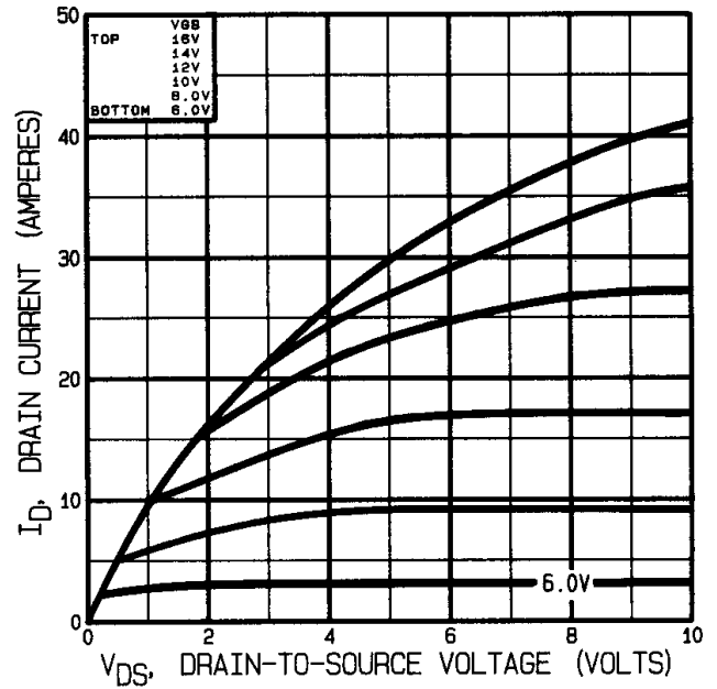
Fig 12. Typical Output Characteristics Post-Irradiation 1 Mega Rads (Si)
