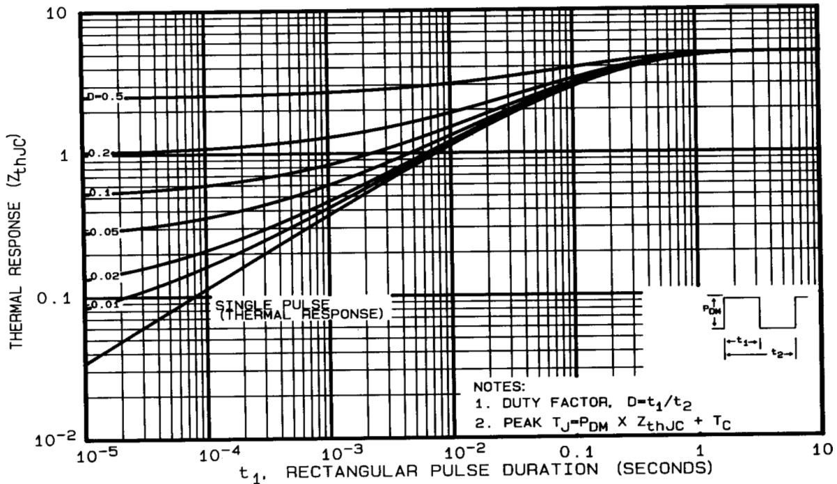
Fig 27. Maximum Effective Transient Thermal Impedance, Junction-to-Case
