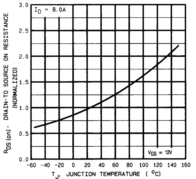
Fig 20. Normalized On-Resistance Vs. Temperature
