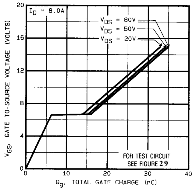
Fig 22. Typical Gate Charge Vs. Gate-to-Source Voltage
