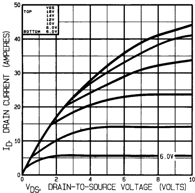
Fig 15. Typical Output Characteristics Post-Irradiation 300K Rads (Si)
