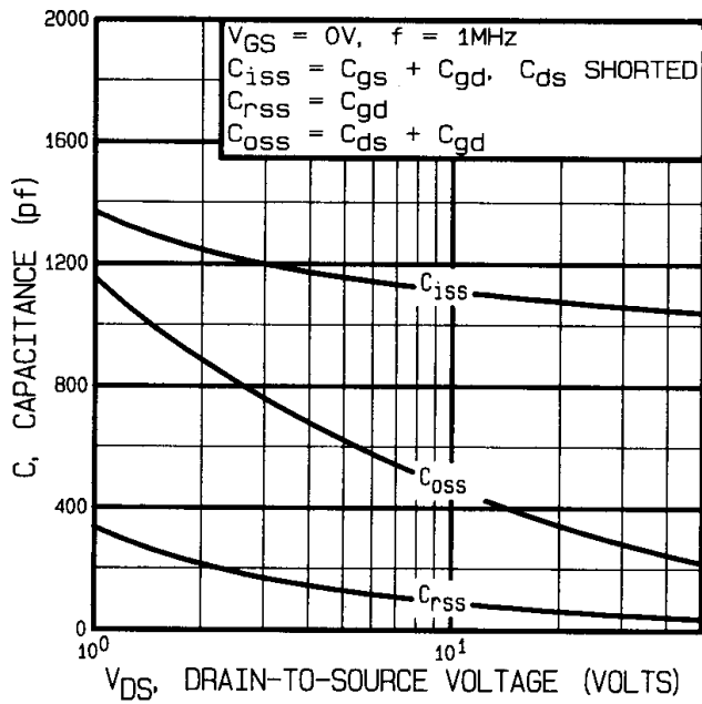
Fig 21. Typical Capacitance Vs. Drain-to-Source Voltage
