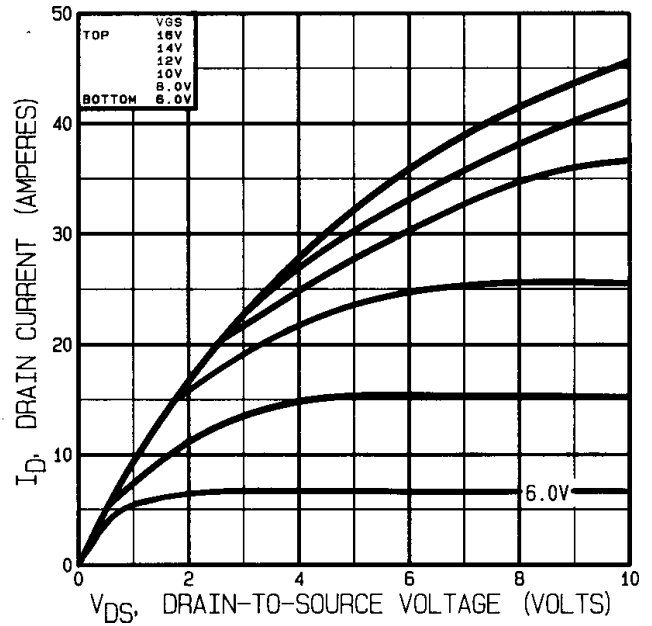
Fig 14. Typical Output Characteristics Post-Irradiation 100K Rads (Si)
