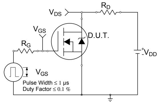
Fig 26a. Switching Time Test Circuit
