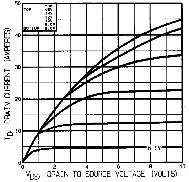
Fig 10. Typical Output Characteristics Post-Irradiation 100K Rads (Si)
